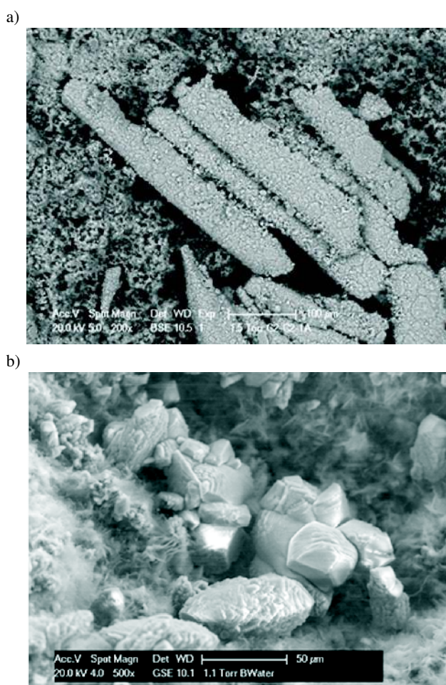
Fig. 7. ESEM photographs showing self-healing activity in bacteria-based concrete specimens. Larger (50–500 \mu\text{m} -sized) calcium carbonate-based precipitates (plate-like, left picture; robust-spherical, right picture) produced by concrete incorporated bacteria on the surface of cracks. Scale bars: left picture 100 \mu\text{m} , right picture 50 \mu\text{m} . (Photographs: ArjanThijssen, Microlab – TU Delft)
