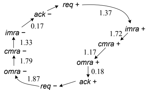
Fig. 15: Speed performance, ns
