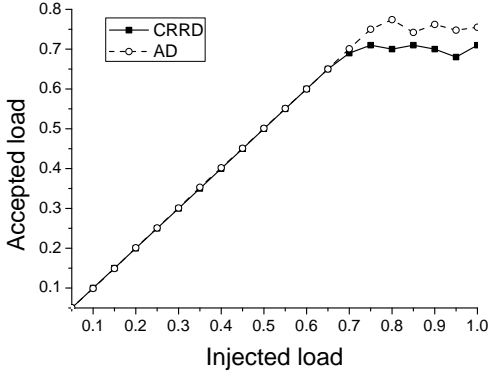
(b) Switch throughput
