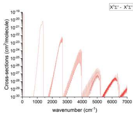
Fig. 11 Overview of the calculated X^1\Sigma^+ state rotation-vibration absorption spectrum of PN at T = 2000\text{ K} with a Gaussian line profile of \text{HWHM} = 1\text{ cm}^{-1} .
