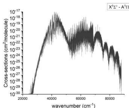
Fig. 12 Calculated absorption spectra of the A^1\Pi - X^1\Sigma^+ system at 2000\text{ K} with a Gaussian profile of \text{HWHM} = 1\text{ cm}^{-1} .
