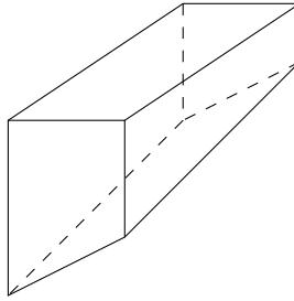
FIGURE 1. Moment polytope for D_3 .
