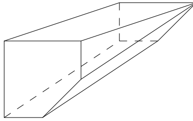
FIGURE 2. Moment polytope for Y_3 .
