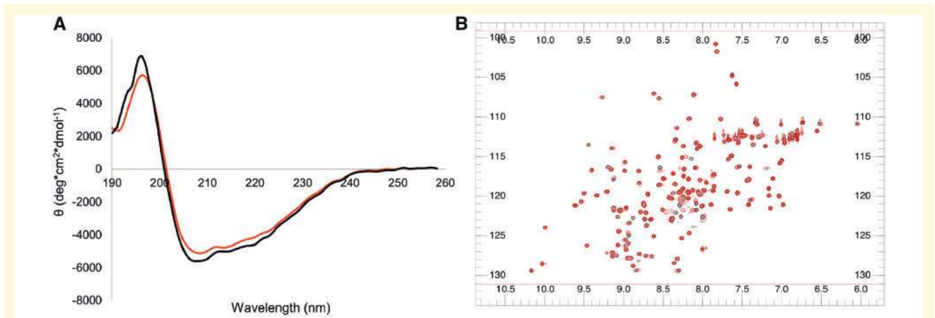
Figure 2 Structural comparison of the wild-type and K181E tandem RRM domains. (A) CD spectra acquired at room temperature, indicating almost complete overlap in their secondary structure. (B) Superposition of heteronuclear single quantum coherence (HSQC) experiments showing that the two variants have nearly identical NMR spectra. Black = wild-type RRM1-2; red = K181E RRM1-2.
