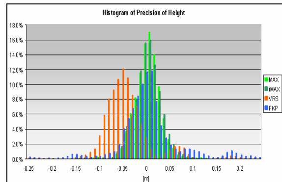
Figure 7. Height histogram from different network RTK corrections
