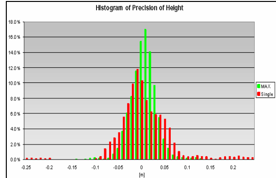
Figure 6. Height histogram from single baseline and MAX corrections
