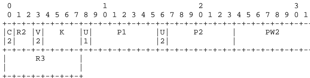
Figure 5: PLC Information Field (PC)
