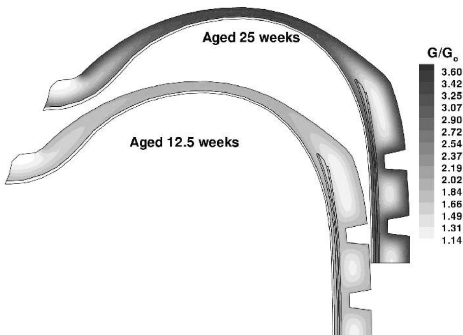
FIG. 6. — Distribution of changes in rubber modulus with oxidation at 70 °C. The lack of change in modulus in the thick sections of tread indicates oxygen starvation in this region. Note that the skim and wedge rubber is oxidizing at 70 °C.
