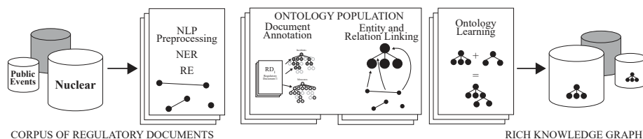
Fig. 2: Natural language processing pipeline that starts with a corpus of regulatory documents (safety instructions, compliance documents, manuals). Via various steps of information extraction and processing a corpus with rich semantic annotation is created. The original data is enriched by semantic information that can be exploited to support users in their search and decisions for instance by recommending and linking related semantic concepts described in other parts of the corpus.
