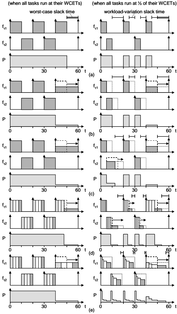
Figure 3: Slack times and voltage scheduling methods. (a) No voltage scheduling, (b) voltage scheduling in [4]-[6], (c) voltage scheduling in [7], (d) voltage scheduling in [7] (4 timeslots), and (e) proposed voltage scheduling (4 timeslots), where f_{\tau_i} and P denote clock frequency of task \tau_i and power consumption of processor, respectively.
