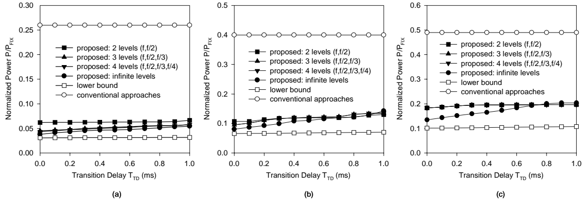
Figure 5: Normalized power consumption for (a) MPEG4, (b) MPEG-2, and (c) VSELP.
