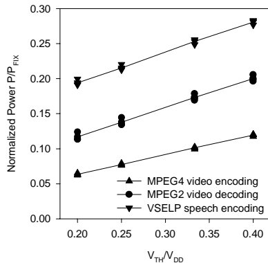
Figure 6: Power consumption for various V_{TH} and V_{DD} .
