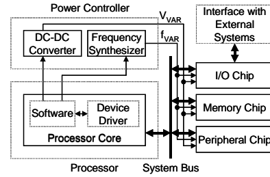
Figure 2: Proposed DVS system architecture.
