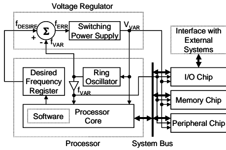
Figure 1: Conventional DVS system architecture.
