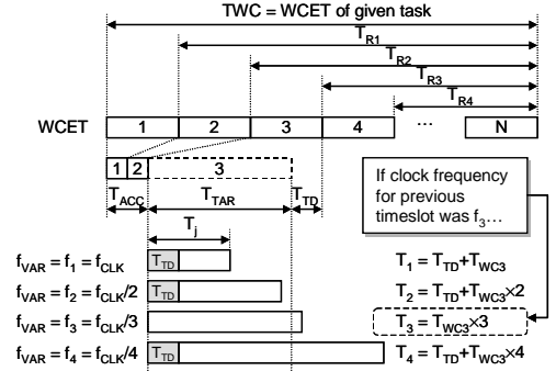
Figure 4: Determination of clock frequency.
