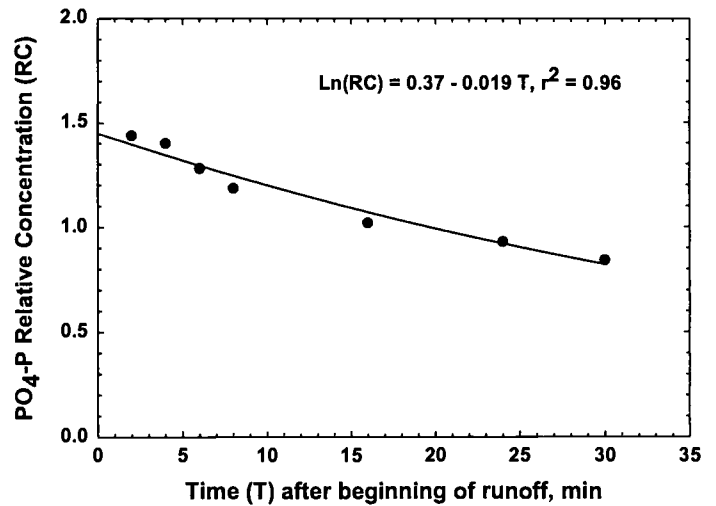
Figure 4. Relationship Between Runoff Ortho-Phosphorus (PO 4 -P) Relative Concentration and Timing of Sample Collection. The filled circles represent means of data, and the line represents the fitted curve.
