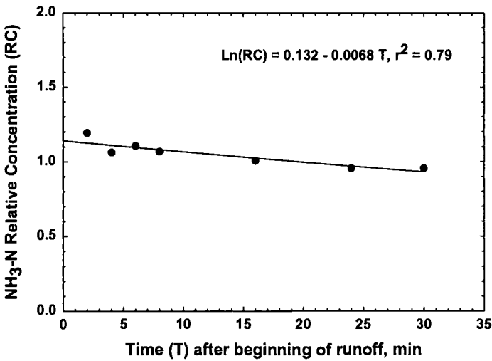
Figure 2. Relationship Between Runoff Ammonia Nitrogen (NH 3 -N) Relative Concentration and Timing of Sample Collection. The filled circles represent means of data, and the line represents the fitted curve.
