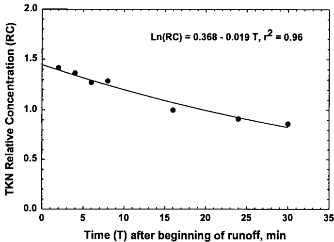
Figure 3. Relationship Between Runoff Total Kjeldahl Nitrogen (TKN) Relative Concentration and Timing of Sample Collection. The filled circles represent means of data, and the line represents the fitted curve.
