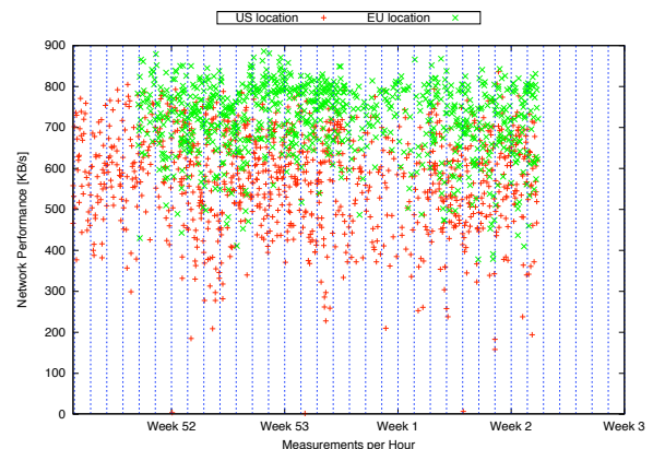
Figure 4: EC2: Network perf., \bar{x} =640, COV: 0.19
