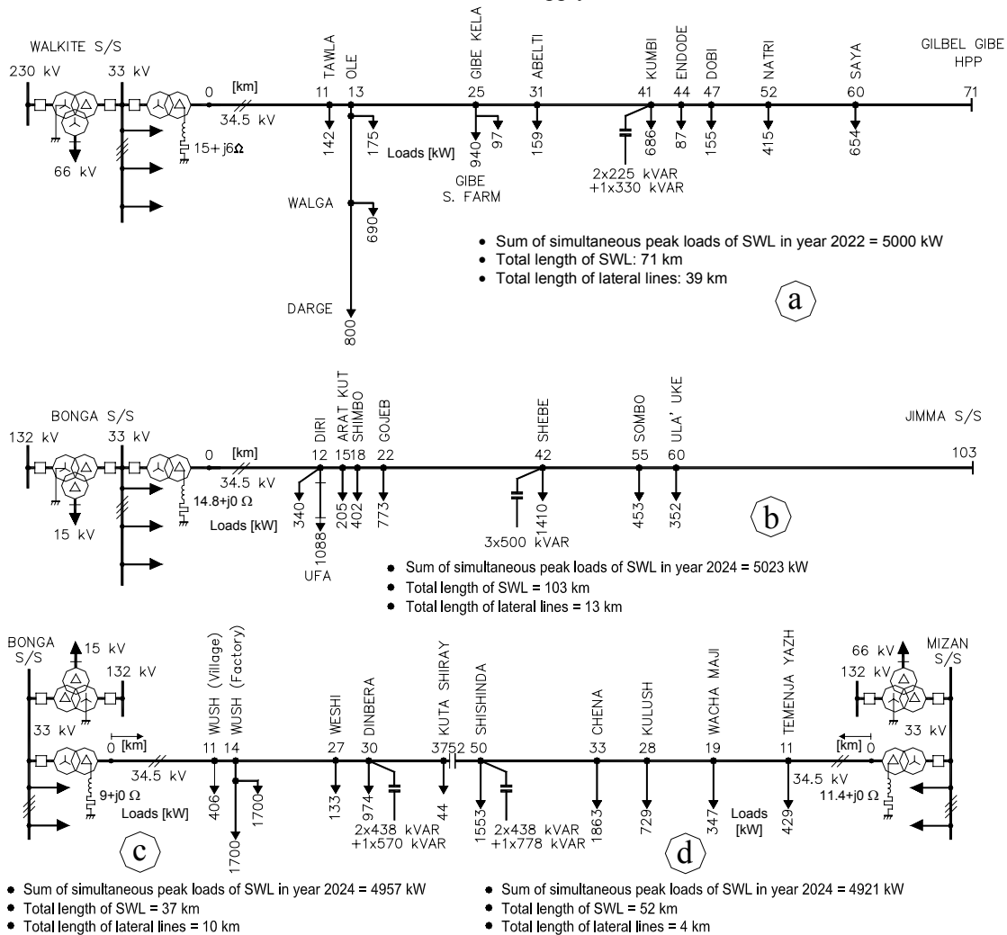
Fig. 4- Single-line diagrams of 34.5 kV “3-Phase” SWSs under construction in Ethiopia
