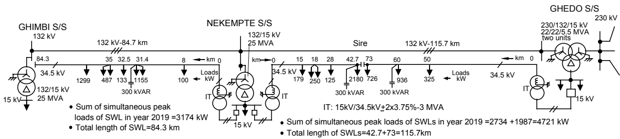
Fig. 3 - Single-Phase Earth-Return SWLs in operation on the Ghedo-Nekempte-Ghimbi 132 kV lines
