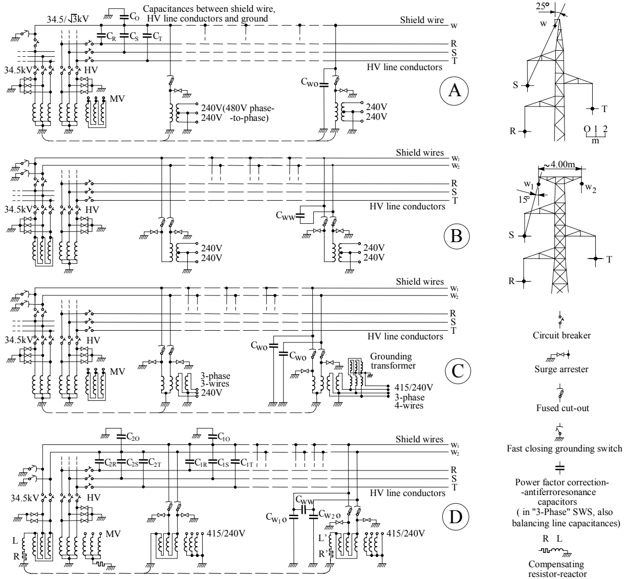
Fig. 1- SWSs applicable to a HV ( V_n \geq 115 kV) single-circuit line: A = Single-Phase Earth-Return (typical line tower is shown on top right); B = Single-Phase Metallic-Return; C = “V” SWS; D = “3-Phase” SWS (typical line tower for SWSs B, C and D is shown on middle right).
