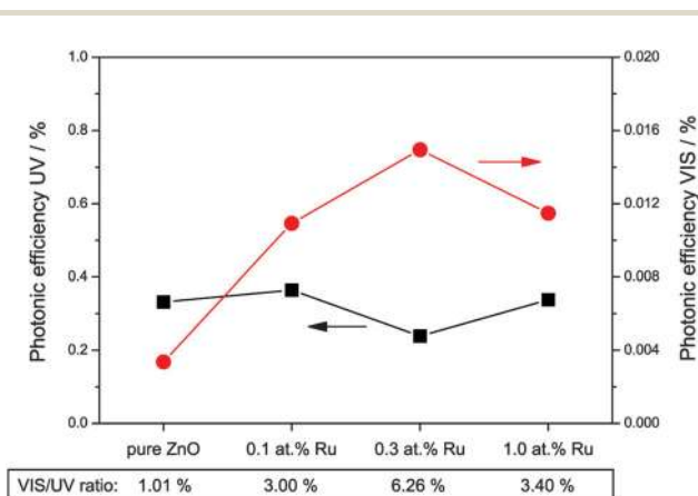
Fig. 9 Photonic efficiencies of hydrogen peroxide formation in the presence of a hole scavenger and under illumination with ultraviolet (black squares, left scale) or visible (red dots, right scale) light. Additionally, the ratio of visible to ultraviolet efficiency is given at the bottom of the figure.
