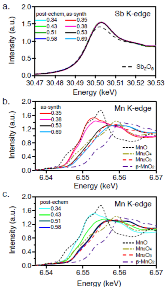
Figure 7. (a) Sb and (b-c) Mn K-edge XAS spectra of rutile alloy \text{Mn}_x\text{Sb}_{1-x}\text{O}_z at a series of Mn concentrations for both as-synthesized and post-electrochemistry films. The reference antimony and manganese oxides with known oxidation states are shown in dashed lines.
