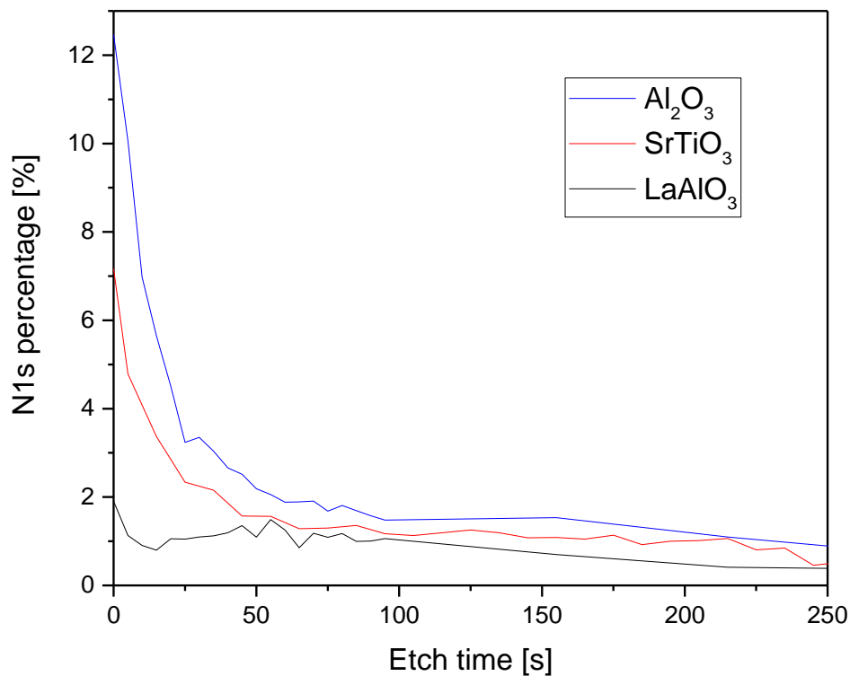
Figure 6. XPS depth profile of N-TiO 2 thin films doped via ammonolysis on differing substrates (Al 2 O 3 , SrTiO 3 , LaAlO 3 ).
