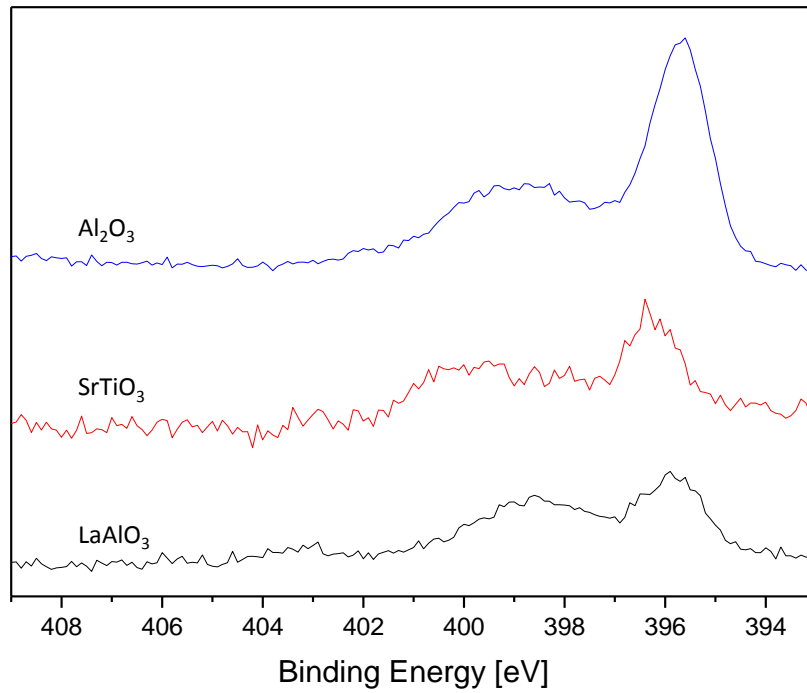
Figure 5. Photoemission spectra of the N 1s core lines in the films of epitaxial TiO 2 on various substrates doped via ammonolysis. Intensities of peaks are concordant with depth profile results (Fig. 6).
