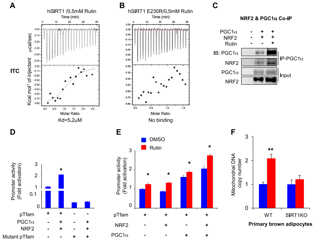
Figure 6. Rutin binds to SIRT1 protein. ITC results show that rutin binds only to WT SIRT1 (A), not to mutant SIRT1 protein (B), in the presence of acetylated peptide substrate p53 in vitro . Coimmunoprecipitation analysis reveals that PGC1 \alpha interacts with NRF2, and this interaction is further enhanced by rutin treatment (C). Rutin treatment further increases PGC1 \alpha - and NRF2-mediated WT, but not NRF2 binding site mutant Tfam luciferase expression (D, E). F) Rutin treatment significantly increased the number of mitochondria in WT but not in SIRT1 KO primary brown adipocytes. Data are means \pm SEM ( n = 3-6 ). * P < 0.05 , ** P < 0.01 vs. control.
