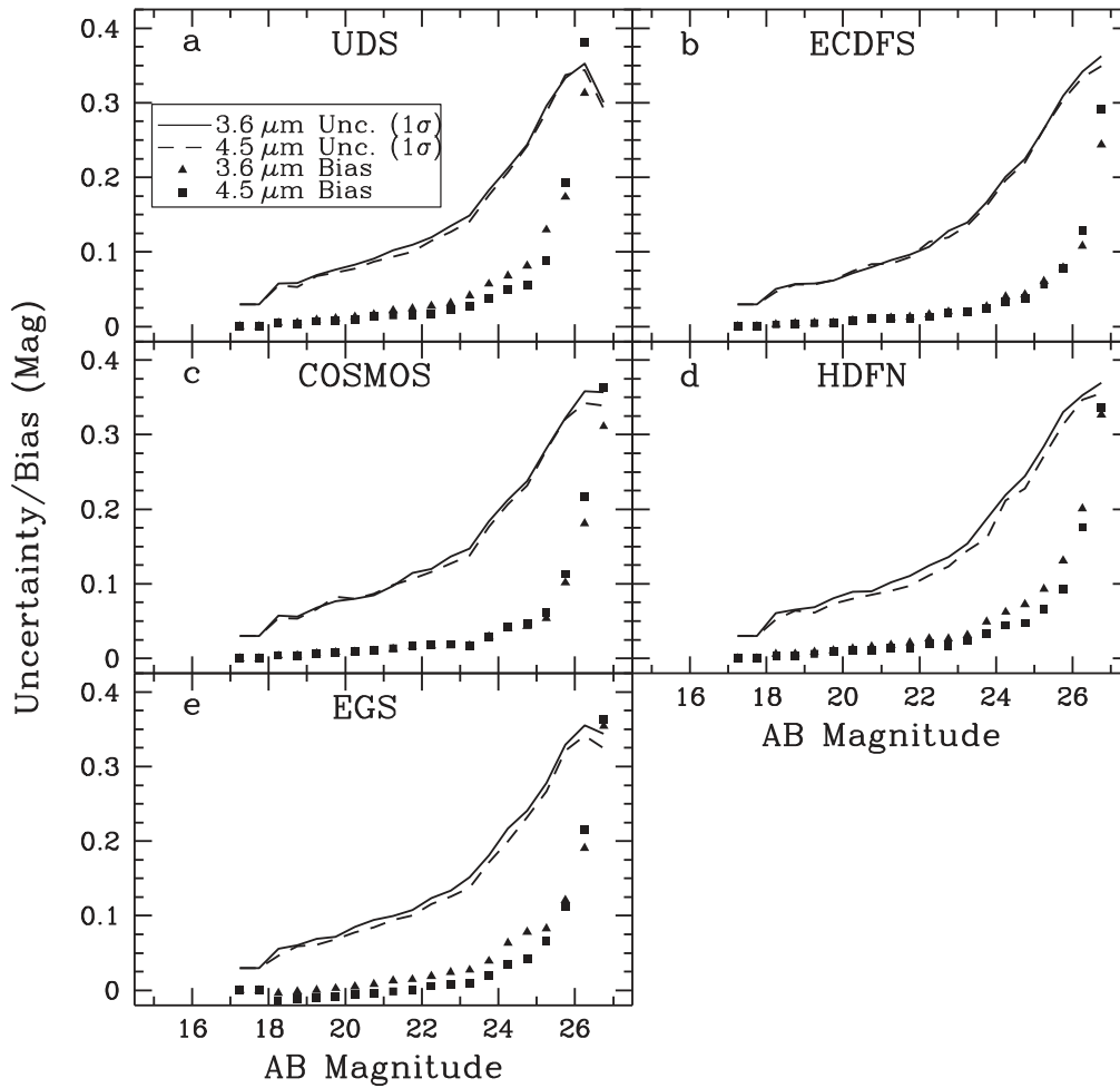
Figure 15. S-CANDELS measurement errors based on photometry of simulated sources as described in Section 3.1. The symbols indicate the measurement bias as a function of apparent magnitude. Positive values indicate that measured values are brighter than the true values. The S-CANDELS catalogs have been corrected for this bias. The solid and dashed lines indicate the 1\sigma measurement uncertainty at 3.6 and 4.5 \mu\text{m} , respectively. The lower limit of 0.03 mag on the measurement uncertainties reflects the uncertainty in the IRAC absolute calibration.
