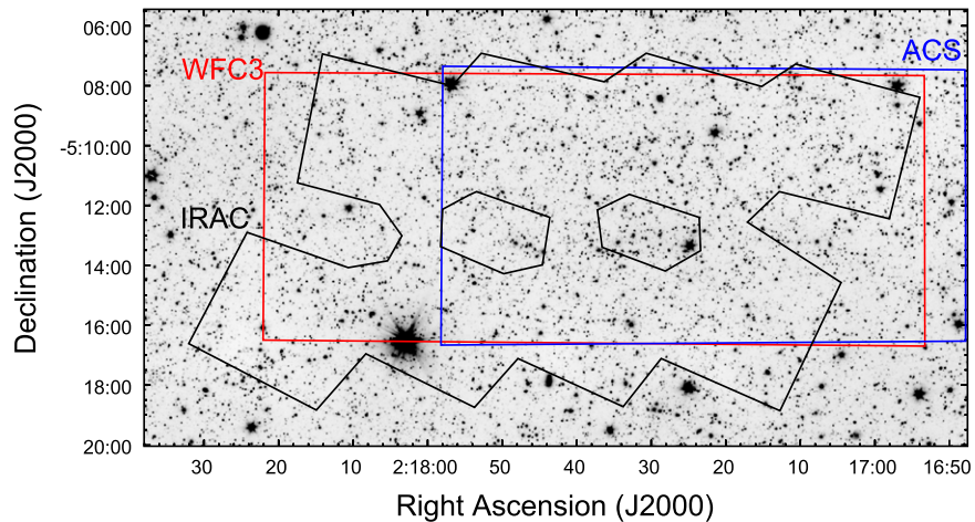
Figure 3. Full-depth S-CANDELS 3.6 \mu\text{m} mosaic in the UDS field, including exposures from the cryogenic mission and SEDS. The image stretch ranges from -0.01 (white) to 0.05 \text{ MJy sr}^{-1} (black). The minimum total exposure time in the field shown is 12 hr. The black polygons indicate where the total IRAC integration reaches 50 hr. The six-sided black polygons in the field center enclose regions where the coverage grades down to the 12 hr SEDS depth. The red and blue rectangles respectively indicate the extent of the HST /WFC3 and ACS imaging from CANDELS (Grogin et al. 2011; Koekemoer et al. 2011).
