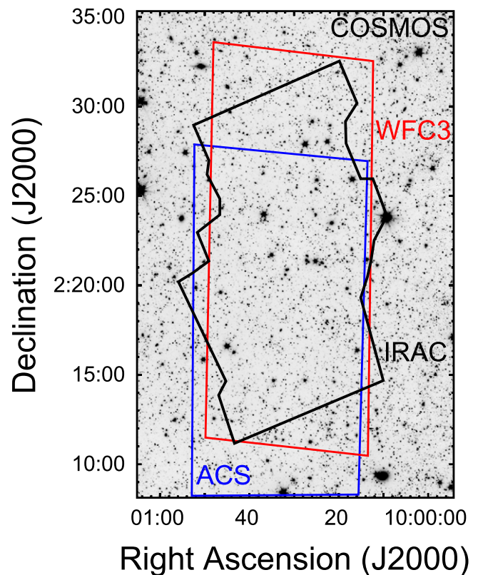
Figure 7. Total S-CANDELS 3.6 \mu\text{m} mosaic in the COSMOS field including all observations from SEDS and the cryogenic mission (Table 1). The image stretch ranges from -0.01 (white) to 0.05 \text{ MJy sr}^{-1} (black). The black polygon approximately indicates the area covered by at least 50 hr of integration time. All of the field shown is covered by at least 12 hr total integration time. The red line encloses the region covered by the CANDELS WFC3 observations, and the blue line encloses the region observed by the CANDELS parallel ACS exposures.
