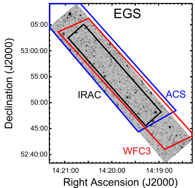
Figure 11. Total S-CANDELS 3.6 \mu\text{m} mosaic of the EGS field. The deepest coverage, at least 50 hr total integration time, lies within the black rectangle. The stretch ranges from -0.01 to 0.05 \text{ MJy sr}^{-1} . Outside the black rectangle the 3.6 \mu\text{m} integration time is at least 12 hr. The blue and red polygons respectively indicate the approximate locations of the CANDELS ACS and WFC3 coverage.
