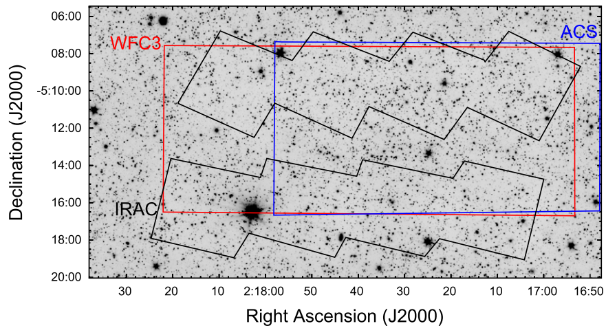
Figure 4. Same as Figure 3, but showing the S-CANDELS 4.5 \mu\text{m} mosaic of the UDS. The stretch ranges from -0.01 to 0.05 \text{ MJy sr}^{-1} .
