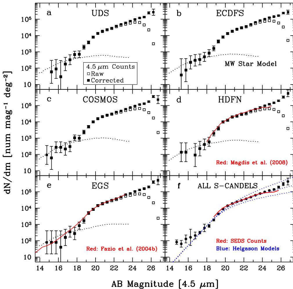
Figure 18. Differential counts in the five S-CANDELS fields at 4.5 \mu\text{m} . The meanings of the symbols are the same as in Figure 17. The Milky Way Star Models shown are those for DIRBE at 4.9 \mu\text{m} , from Arendt et al. (1998), Wainscoat et al. (1992), and Cohen et al. (1993, 1994, 1995).
