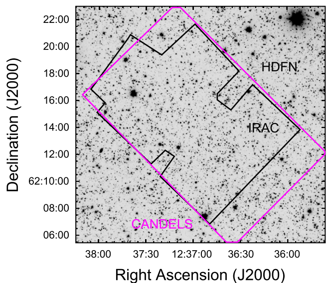
Figure 9. Total SCANDELS IRAC 3.6 \mu\text{m} mosaic in the HDFN. The black polygon indicates approximately where the total 3.6 \mu\text{m} integration time, which includes observations from the cryogenic mission (i.e., GOODS), rises to at least 50 hr. The magenta rectangle indicates the coextensive HST /WFC3 +ACS footprint from CANDELS. The stretch ranges from -0.01 to 0.05 \text{ MJy sr}^{-1} .
