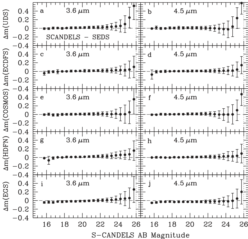
Figure 16. Comparison of S-CANDELS and SEDS photometry at 3.6 and 4.5 \mu\text{m} . Symbols indicate the mean differences for measurements made in 2'' diameter apertures within bins 0.5 mag wide. Positive-valued differences mean sources appear brighter in SEDS than in S-CANDELS on average. All error bars are 1\sigma . Vertical dotted lines indicate the SEDS 3\sigma sensitivity limits. The comparison was made after both photometric datasets were corrected to total magnitudes by compensating for empirically determined aperture losses and biases.
