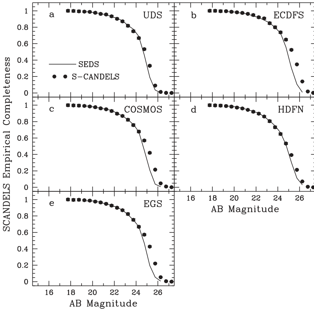
Figure 14. Completeness in the S-CANDELS fields estimated by Monte Carlo simulations as described in Section 3.1. Symbols indicate the completeness measured in bins of width 0.5 mag within the S-CANDELS fields shown in Figures 3–12 where the depth of coverage was at least 12 hr; the mean coverage was by design significantly higher (Figure 2). The completeness measured for SEDS, specifically coverage of at least 10 ks total exposure time in the wider-but-shallower SEDS mosaics from Ashby et al. (2013a), is indicated with the black line. In both cases the values given are by-field averages. The completeness in any particular small region depends on the actual integration time achieved there and on the highly variable local source confusion.
