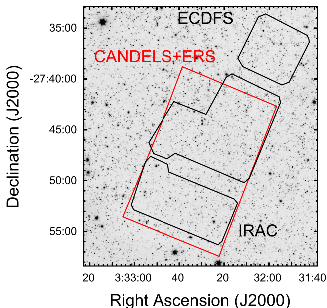
Figure 6. Same as Figure 5, but showing the full-depth 4.5 \mu\text{m} mosaic of the ECDFS including all SEDS and cryogenic imaging by IRAC. The stretch ranges from -0.01 to 0.05 \text{ MJy sr}^{-1} .
