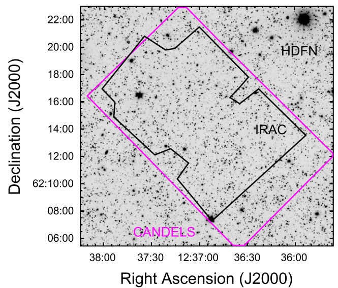
Figure 10. As Figure 9, but for the 4.5 \mu\text{m} observations. The stretch ranges from -0.01 to 0.05 \text{ MJy sr}^{-1} .
