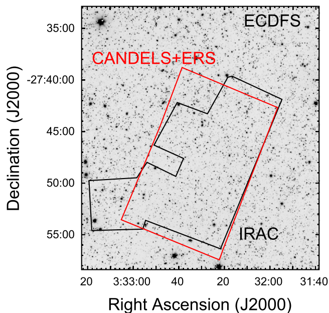
Figure 5. Full-depth SCANDELS 3.6 \mu\text{m} mosaic of the ECDFS. The stretch ranges from -0.01 to 0.05 \text{ MJy sr}^{-1} . The black polygon encloses a region where the depth of coverage is a minimum of 50 hr. The red rectangle indicates the portion of the field covered by the HST CANDELS and ERS programs.
