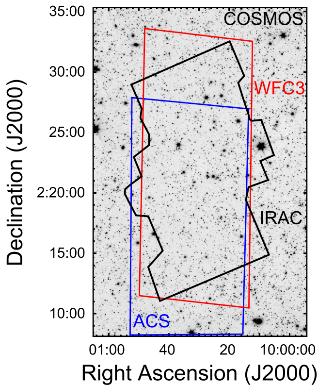
Figure 8. Same as Figure 7, but showing the full-depth 4.5 \mu\text{m} mosaic in the COSMOS field. The stretch ranges from -0.01 to 0.05 \text{ MJy sr}^{-1} .
