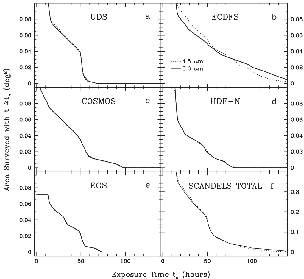
Figure 2. Cumulative area coverage as a function of exposure time for S-CANDELS, including other, earlier observations (Table 1). The solid and dotted lines correspond, respectively, to the 3.6 and 4.5 \mu\text{m} bands. Panel (f) shows the coverage summed over all five S-CANDELS fields. The nominal S-CANDELS depth was 50 hr.
