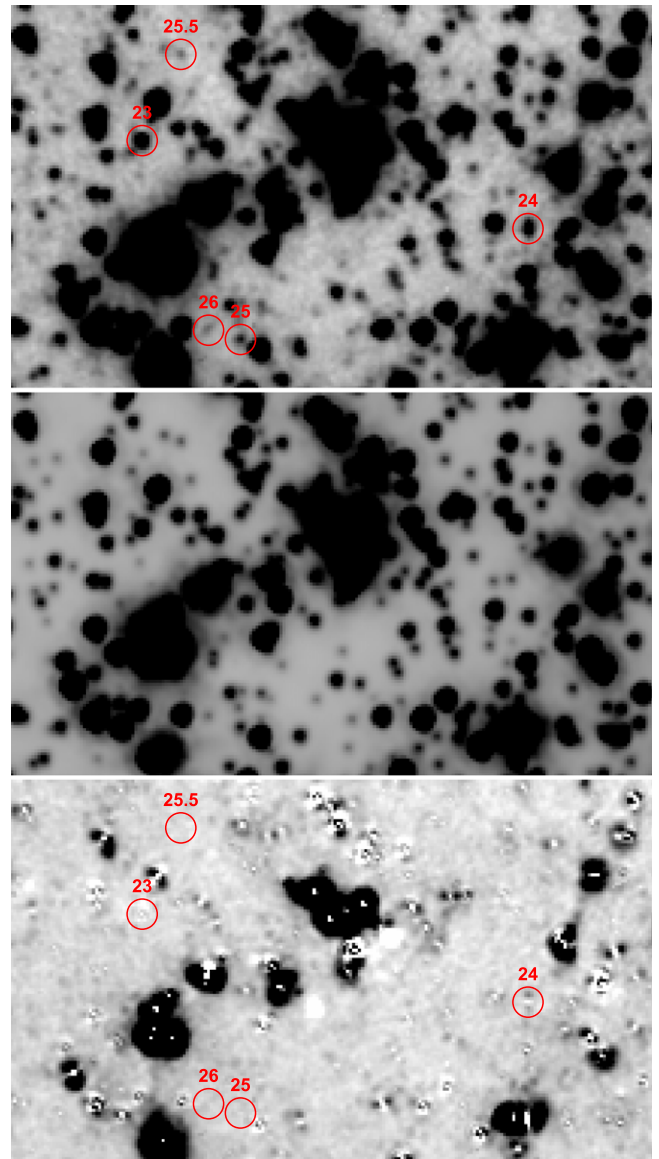
Figure 13. Illustration of StarFinder source extraction. These negative images show a 2.1 \times 1.2 region of the 3.6 \mu\text{m} S-CANDELS ECFDS mosaic; the other S-CANDELS band and fields behave in a similar way. The linear stretch ranges from -0.001 (white) to 0.004 \text{ MJy sr}^{-1} (black) throughout. Top: the IRAC 3.6 \mu\text{m} mosaic created by IRACProc . Red circles are placed around sources with AB magnitudes as shown. Center: the corresponding StarFinder model image. Bottom: the residual image obtained after the detected sources are removed.
