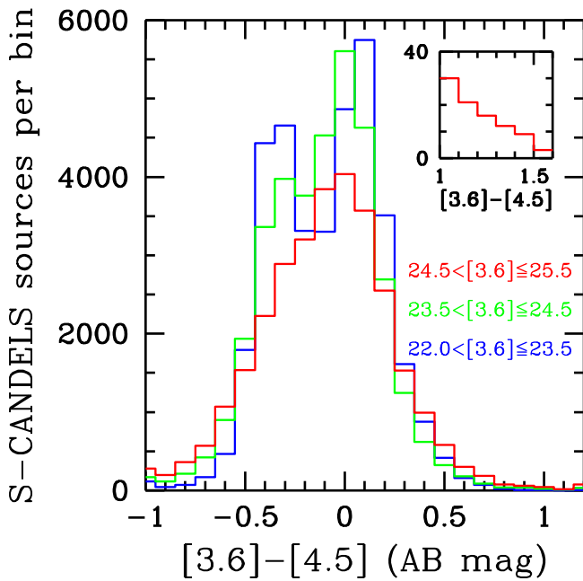
Figure 19. Histograms of S-CANDELS sources in three magnitude bins as indicated by colors. The inset shows the distribution of the reddest sources in the 24.5 < [3.6] < 25.5 magnitude range. There are 118 sources in this range with [3.6] - [4.5] > 1 of which 27 have [3.6] - [4.5] > 1.6 . Given the photometric uncertainties (Figure 16), the apparent red colors may be due to photometric errors.
