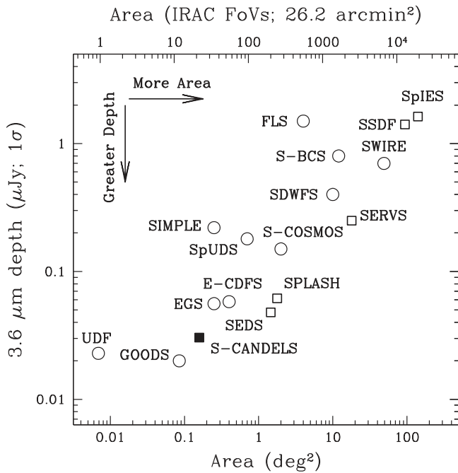
Figure 1. Comparison of measured S-CANDELS 3.6 \mu\text{m} 1\sigma depth and total area (solid square) to other major Spitzer /IRAC extragalactic surveys from the cryogenic mission (circles) and warm mission (squares). The points shown for S-CANDELS, SEDS (Ashby et al. 2013a), SDWFS (Ashby et al. 2009), and SSDF (Ashby et al. 2013b) are based on photometry of simulated sources in mosaic images and therefore account for source confusion. All other points are taken from the online calculator SENS-PET, using the appropriate sensitivities for the cryogenic and warm mission. Low-background conditions were assumed throughout except for SpIES, for which a medium background was (conservatively) assumed. Surveys shown include Great Observatories Origins Deep Survey (GOODS; Giavalisco et al. 2004; Wang et al. 2010; Hathi et al. 2012; Lin et al. 2012), the Extended Groth Strip (EGS; Davis et al. 2007; Bielby et al. 2012), Extended Chandra Deep Field South (E-CDFS; Rix et al. 2004; Castellano et al. 2010), Spitzer Public Legacy Survey of UKIDSS Ultra-deep Survey (SpUDS; Caputi et al. 2011), SCOSMOS ( Spitzer Deep Survey of HST COSMOS 2-Degree ACS Field; Scoville et al. 2007a), Spitzer Extragalactic Representative Volume Survey (SERVS; Mauduit et al. 2012), Blanco Cluster Survey (BCS), Spitzer Wide-area Infrared Extragalactic Survey (SWIRE; Lonsdale et al. 2003, 2004), the Spitzer First Look Survey (FLS; Fang et al. 2004), the Ultra-deep Field (UDF; Labbé et al. 2013), the Spitzer IRAC/MUSYC Public Legacy in E-CDFS (SIMPLE; Damen et al. 2011), Spitzer -IRAC Equatorial Survey (SpIES), and Spitzer Large-area Survey with Hyper-Suprime-Cam (SPLASH). Compared to the analogous Figure 1 of Ashby et al. (2013a), SpIES, SSDF, SERVS, and S-CANDELS have all been updated because they relied on SENS-PET estimates that did not yet account for the slightly reduced sensitivity of IRAC during the warm mission.
