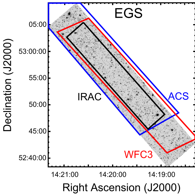
Figure 12. Same as Figure 11, but for the total S-CANDELS 4.5 \mu\text{m} mosaic of the EGS field. The stretch ranges from -0.01 to 0.05 \text{ MJy sr}^{-1} .
