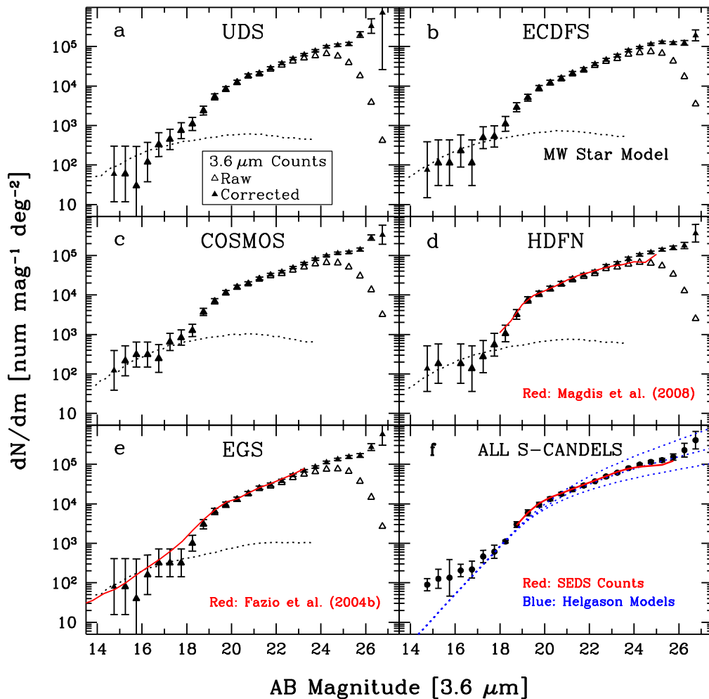
Figure 17. Differential 3.6 \mu\text{m} counts in the five S-CANDELS fields. Open symbols show the raw counts, while solid symbols indicate the counts corrected for incompleteness on the basis of simulated detections as described in Section 3.1. Error bars represent the Poisson statistics only in panels (a)–(e). The solid red lines in panels (d) and (e) indicate the incompleteness-corrected counts measured in the HDFN by Magdis et al. (2008) and in the EGS by Fazio et al. (2004b), respectively. The dotted lines in panels (a)–(e) show the expected counts arising from Milky Way stars, based on the DIRBE Faint Source Model at 3.5 \mu\text{m} (Wainscoat et al. 1992; Cohen et al. 1993, 1994, 1995; Arendt et al. 1998). Panel (f) shows the area-weighted mean counts for all of S-CANDELS together with predicted counts from Helgason et al. (2012). The upper and lower blue dotted lines indicate the Helgason et al. high-faint-end and low-faint-end luminosity function models, i.e., models in which the slopes of the faint end of the luminosity functions were respectively set to \alpha = -1.2 and -0.8 . The middle blue dashed line indicates the so-called “default” model, obtained by averaging the high-faint-end and low-faint-end models. The SEDS source counts are shown in red.
