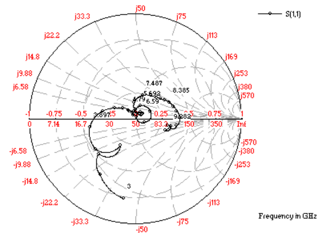
Fig 8: Smith Chart
