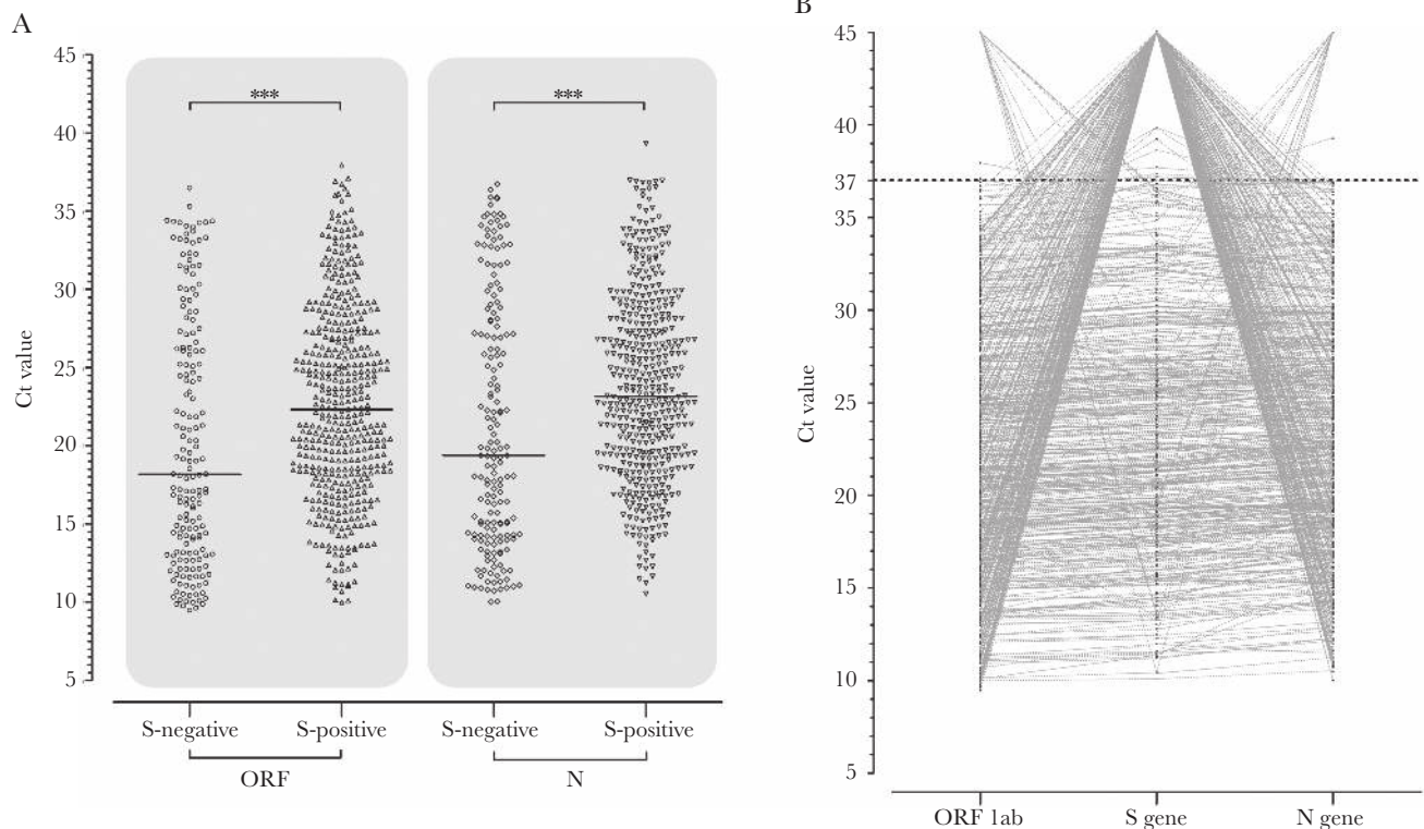
Figure 2. A, Scatter plot of the population of S gene-negative (SGTF)/S-gene positive Cts within corresponding ORF1ab and N-gene positive samples. Median Ct is shown by a black horizontal bar. Above both plots the results of Mann-Whitney U tests for significant differences are shown; *** P < .0001 . B, Scatter plot of viral gene Ct values for individual positive samples. The horizontal dotted line at Ct 37 represents the threshold for a target-negative result as defined for clinical interpretation in the TaqPath instructions for use. The class of target-undetectable results have a nominal value of Ct 45 assigned (described in “Methods” section). Each set of 3 Ct values for a sample is linked by a grey dotted line. Abbreviations: Ct, cycle threshold; N, nucleocapsid; ORF1ab, open reading frame 1ab; S, spike.
