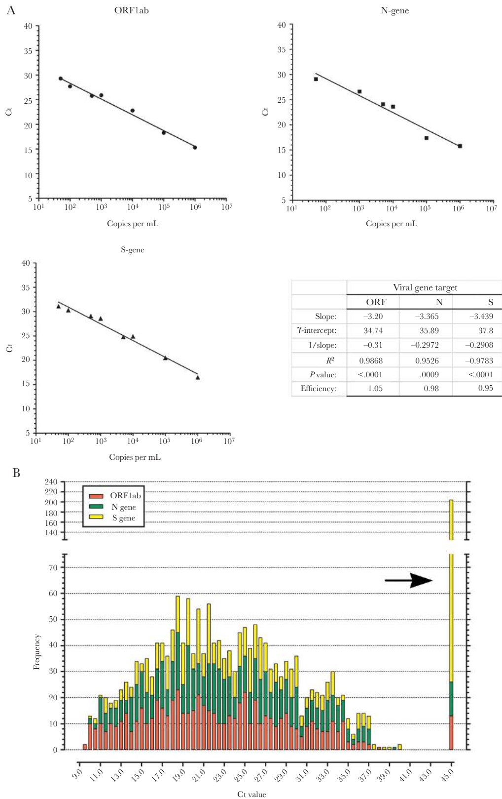
Figure 1. A, Verification data for TaqPath RT-PCR test using the Qnostics external quality assurance dilution series SCV2AQP01-A. Linear regression plots for ORF1ab, N, and S gene targets are shown with regression data including efficiency calculations for each gene target. B, Stacked bar frequency diagram showing the proportional relationship between all 3 viral gene targets detected by RT-qPCR, at each Ct value across the range. Y-axis is divided into a low sample frequency range of 0–75 and a high range of 130–240. Arrow shows gene target failures for S, N, and ORF1ab. Abbreviations: Ct, cycle threshold; N, nucleocapsid; ORF1ab, open reading frame 1ab; RT-qPCR, reverse transcription quantitative polymerase chain reaction; S, spike.
