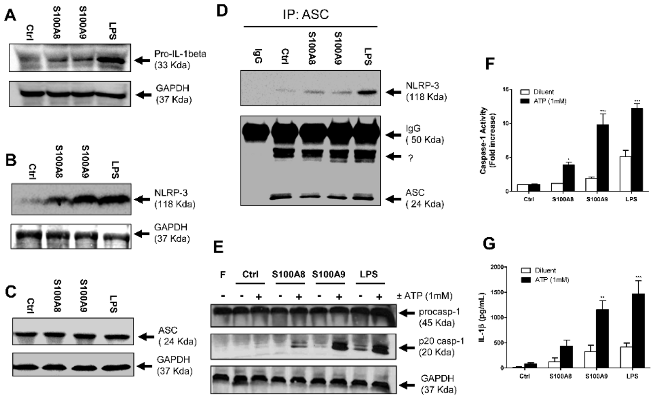
Figure 6. S100A8 and S100A9 regulate the NLRP3 inflammasome. Cells were incubated for 4 h with S100A8 (10 \mu\text{g/ml} ), S100A9 (10 \mu\text{g/ml} ), LPS (1 \mu\text{g/ml} ), or the equivalent volume of buffer (Ctrl). For some experiments, ATP (1 mM) was added for 30 min (D–G). Cells were harvested and lysed with Laemmli's buffer for immunoblotting of pro-IL-1 \beta (A), NLRP3 (B), ASC (C) or caspase-1 (E). Cells were lysed with caspase-1 lysis buffer for the caspase assay (F). ASC immunoprecipitates were loaded on SDS-PAGE for NLRP-3 and ASC western blot analysis (D). Supernatants were harvested before performing IL-1 \beta ELISA (G). Results are from one experiment that is representative of at least three others (A–E). Data are the mean \pm SEM of three experiments performed on cells from different donors (F–G). ?, non-specific band (as indicated in the manufacturer's datasheet). * p \leq 0.05 , ** p \leq 0.01 , *** p \leq 0.005 , Dunnett's multiple comparison test. doi:10.1371/journal.pone.0072138.g006
