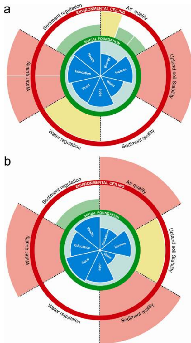
Fig. 5. Safe and just operating spaces mapped for two Chinese regions in 2006. (a) Erhai lake-catchment system, Yunnan Province; (b) Shucheng County, Anhui Province. The figures show the extent to which each region currently meets expected social standards (blue sectors) for an acceptable social foundation (green circle), and the current status of key ecological services/processes (from Figs. 3 and 4): safe (green sectors), cautious (yellow sectors) and dangerous (red sectors). The environmental ceiling (red circle) defines the approximate boundary between sustainable and unsustainable use of ecological processes. The RSJOS exists as a 'doughnut' between the environmental ceiling and social foundation. Data for sediment quality (a) and water regulation (b) unavailable. Note that the relative sizes of green, yellow and red sectors are illustrative: they are not plotted to any scale and are not plotted from the centre of the circles (see text for further explanation). Blank sectors indicate unavailability of data. Ecological data are shown in Figs. 3 and 4, and Tables A.2 and A.4; social data in Tables A.3 and A.5. An additional sector for upland soil stability at Erhai (a) is based on assessment of centennial records (see text and Dearing, 2008). (For interpretation of the references to color in this text, the reader is referred to the web version of the article.)
