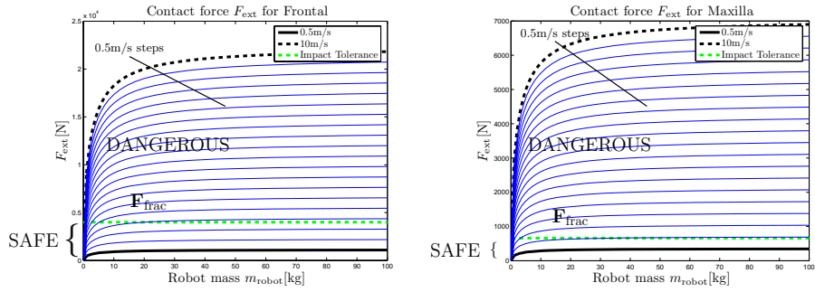
Fig. 3. Contact forces for simulated impacts between a robot and the frontal area (left) and the maxilla (right), showing the dependency on the robot mass and velocity. The impact velocity steps are 0.5m/s. One has to take into consideration that the applied human model is not valid anymore after the fracture occurs. This is discussed in [11].
