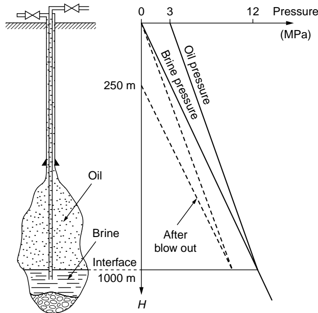
Figure 2 Pressure distribution before and after a blow out. Oil and brine pressures are equal at interface depth; oil pressure is larger at smaller depth. After a blow out (dashed lines), pressures drop as the air/brine interface lowers in the tubing.
