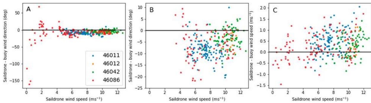
Fig. 5. Sailsdrone minus buoy differences in (a) wind direction, (b) wind direction, and (c) wind speed as a function of wind speed. At low wind speeds, the scatter increases and this only occurred at buoy 46086. Note that (b) is as in (a), but with wind speeds less than 3 \text{ m s}^{-1} removed.
