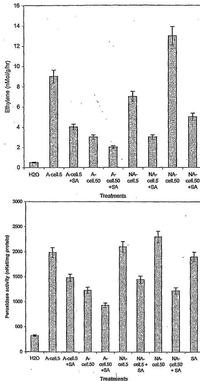
Figure 9. Effect of SA on ethylene content (A) and peroxidase activity (B). Cotyledons were co-infiltrated with SA ( 800 \mu\text{M} ) and cellulase. Ethylene level (A) was measured 24 h after infiltration. Peroxidase activity (B) was measured 72 h later in cotyledons. SA solution was prepared by titration with 0.1 \text{ M} NaOH to a pH value around 7.0. Each value is the mean \pm SE of 10 replicates from different plants.
