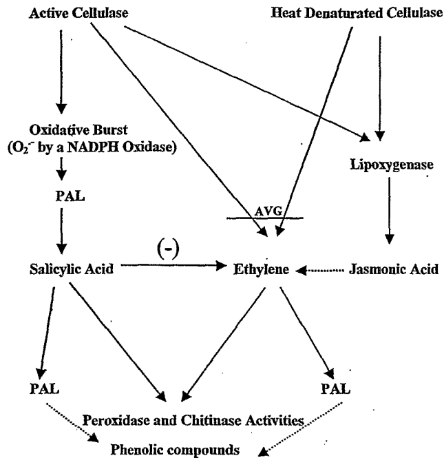
Figure 12. Cellulase-induced signaling pathway in melon cotyledons.
