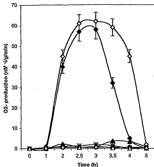
Figure 10. Time course of O_2^{\cdot-} production in cotyledons after A-cell. and NA-cell. infiltration. ●, Control; ◆, A-cell.5; *, A-cell.5 + DPI; ▲, NA-cell.5; ◇, A-cell.50; △, NA-cell.50. Cotyledon discs were incubated in cytochrome C medium, and superoxide anion production was monitored periodically by the reduction of cytochrome C. DPI was added to the reaction buffer just before immersion of cotyledon discs in cytochrome C buffer. Each value is the mean \pm SE of 10 replicates from different plants
