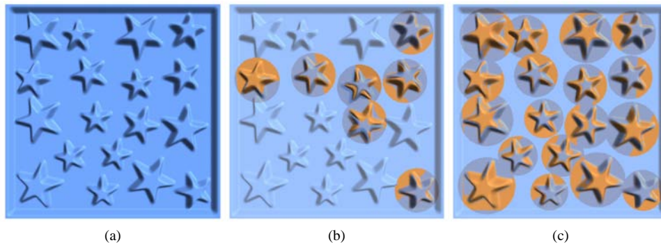
Fig. 20. The stars model (a) consist of 18 stars of three different scales. A medium scale star is used as a query. The result of using spin-images and our method are shown in (b) and (c), respectively. This example illustrates the fact that our method is scale-independent.
