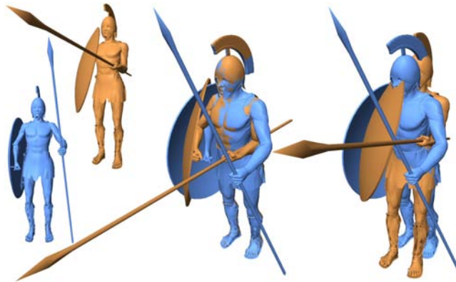
Fig. 13. Model alignment based on global principle component analysis (PCA) (right) and partial matching (left).
