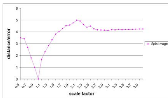
Fig. 19. The L_2 distance between spin-images computed around the same points at different scales and the spin-image at scale 1.0. The graph shows the sensitivity of the spin-image signature to scale.
