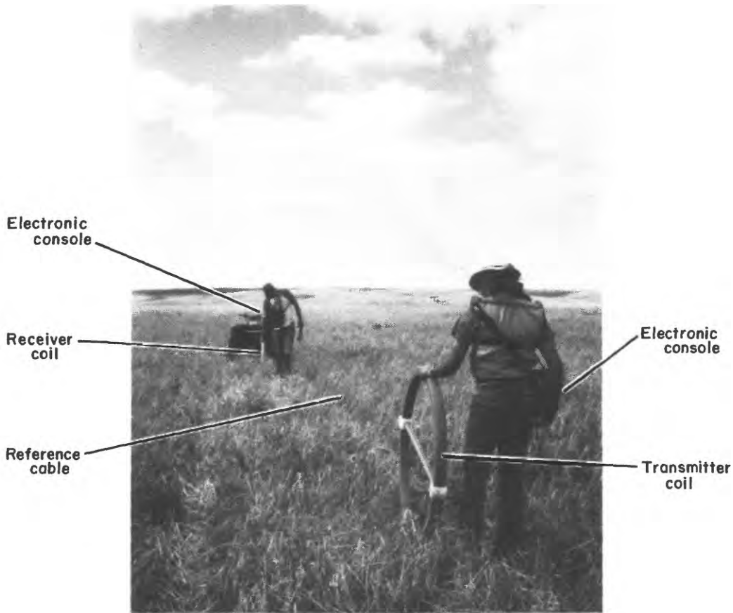
Figure 9. Electromagnetic geophysical equipment in the horizontal-dipole orientation.
