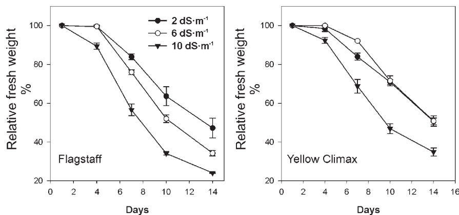
Fig. 1. Relative fresh weight reduction of flowering shoots of marigold Tagetes erecta 'Flagstaff' and 'Yellow Climax' as affected by preharvest irrigation water electrical conductivity (2, 6, 10 dS·m -1 ). Bars represent the SE of the mean (n = 3).
