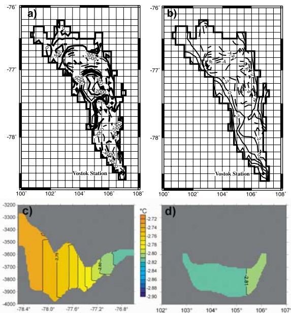
Figure 2. (a) Vertically integrated mass transport stream function ( \text{m}^3 \text{s}^{-1} ) for a freshwater lake. (b) Rates of basal melting (negative) and freezing (positive) ( \text{cm yr}^{-1} ). (c) Meridional potential temperature distribution along 106^\circ\text{E} . (d) Zonal potential temperature distribution along 77^\circ\text{S} . The vertical scale in (c) is about 330-fold, in (d) about 190-fold exaggerated.
