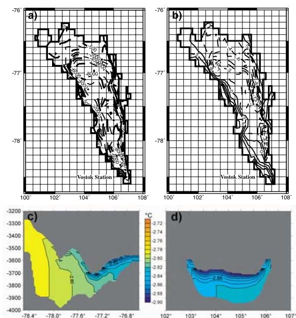
Figure 3. Results for a lake water salinity of 1.2\text{‰} . Captions as in Figure 2.
