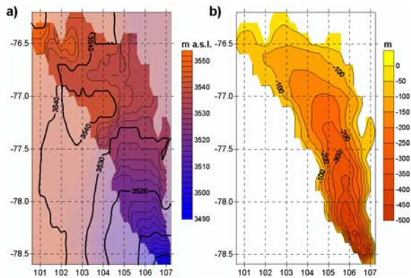
Figure 1. (a) Surface elevation and extent of Lake Vostok derived from airborne radar measurements of the lake edge and ice surface gradient transitions, (b) constructed water depth in the lake relative to the ice sheet base.
