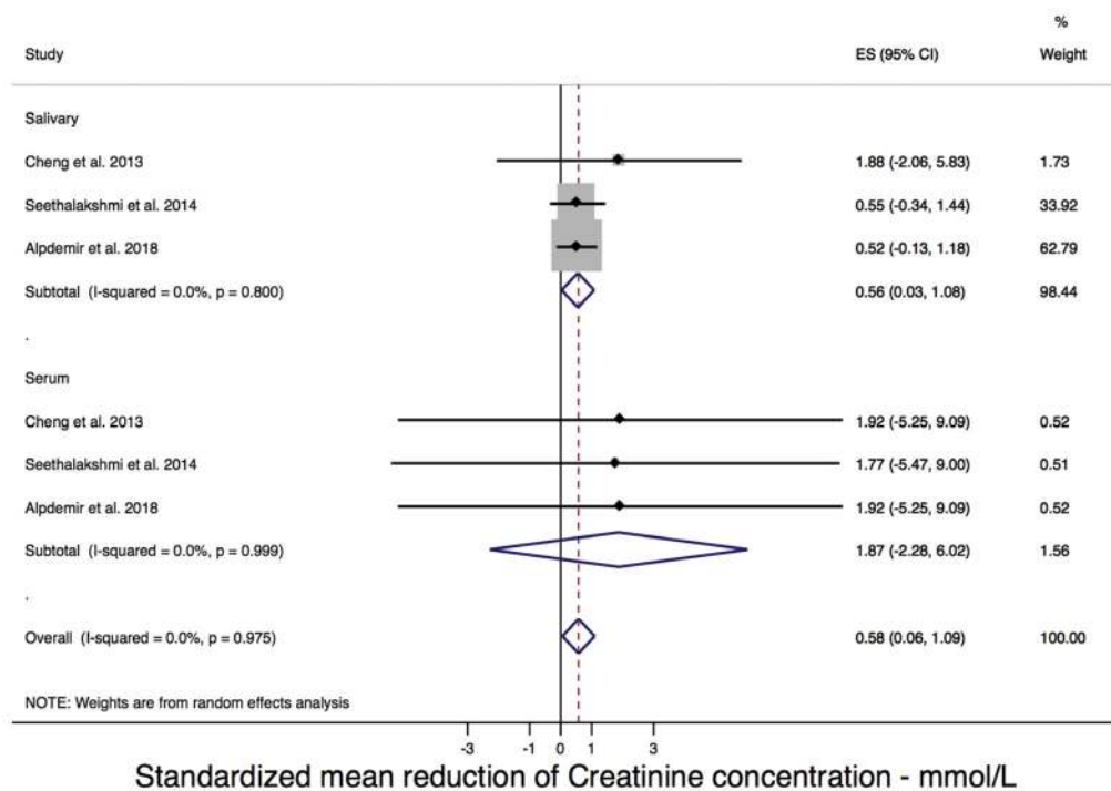
Figure 4A. Forest plot of the subgroup meta-analysis of Hedges standard mean difference (g) of creatinine concentration from pre- to posthemodialysis. Weights are from random effects analysis.
