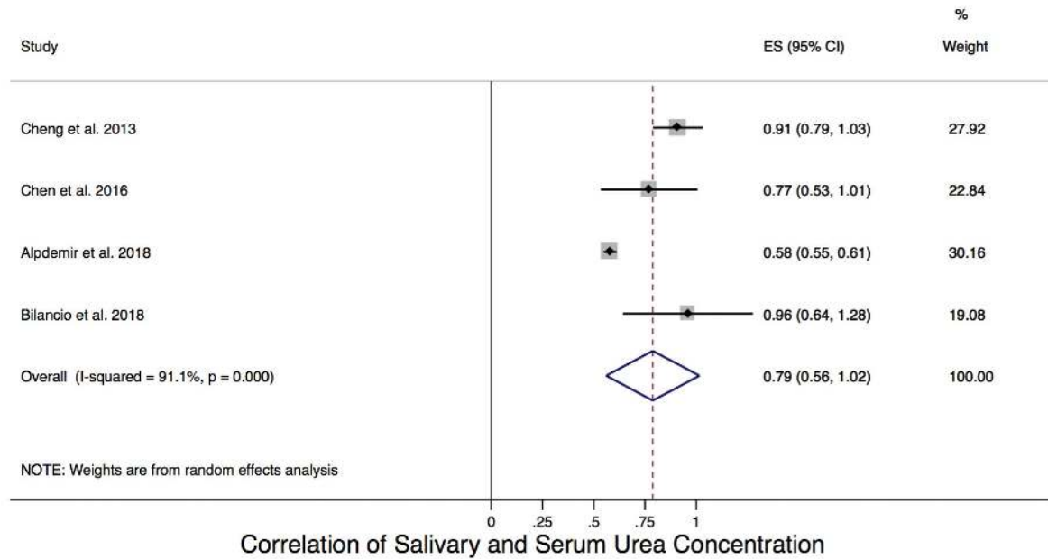
Figure 2A. Forest plot of the correlation between salivary and serum urea concentration. Weights are from random effects analysis.
