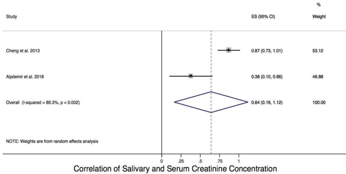
Figure 2B. Forest plot of the correlation between salivary and serum creatinine concentrations. Weights are from random effects analysis.
