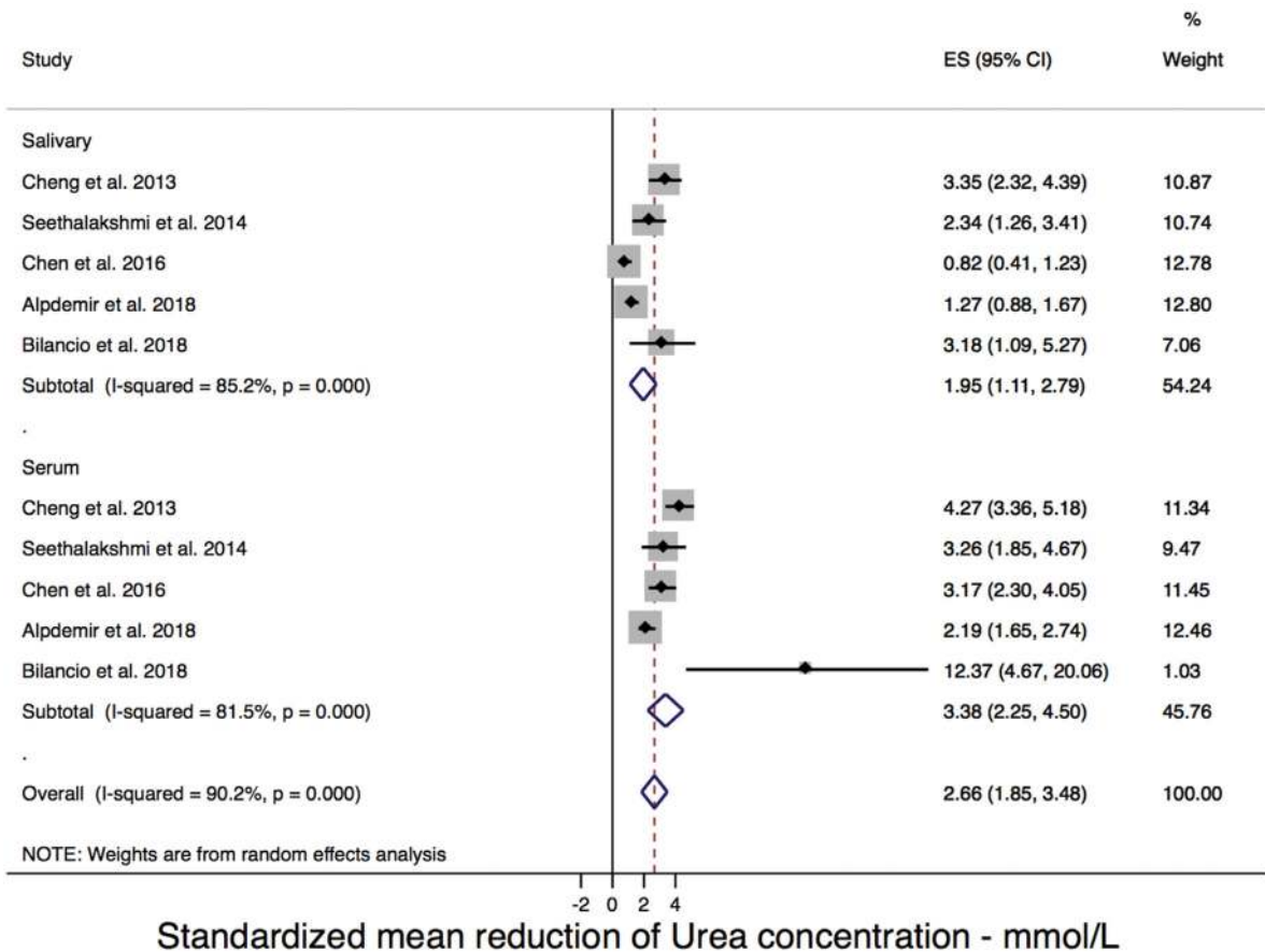
Figure 3A. Forest plot of the difference in urea concentrations from pre- to posthemodialysis meta-analysis of Hedges standard mean difference (g) of urea concentration. Weights are from random effects analysis.
