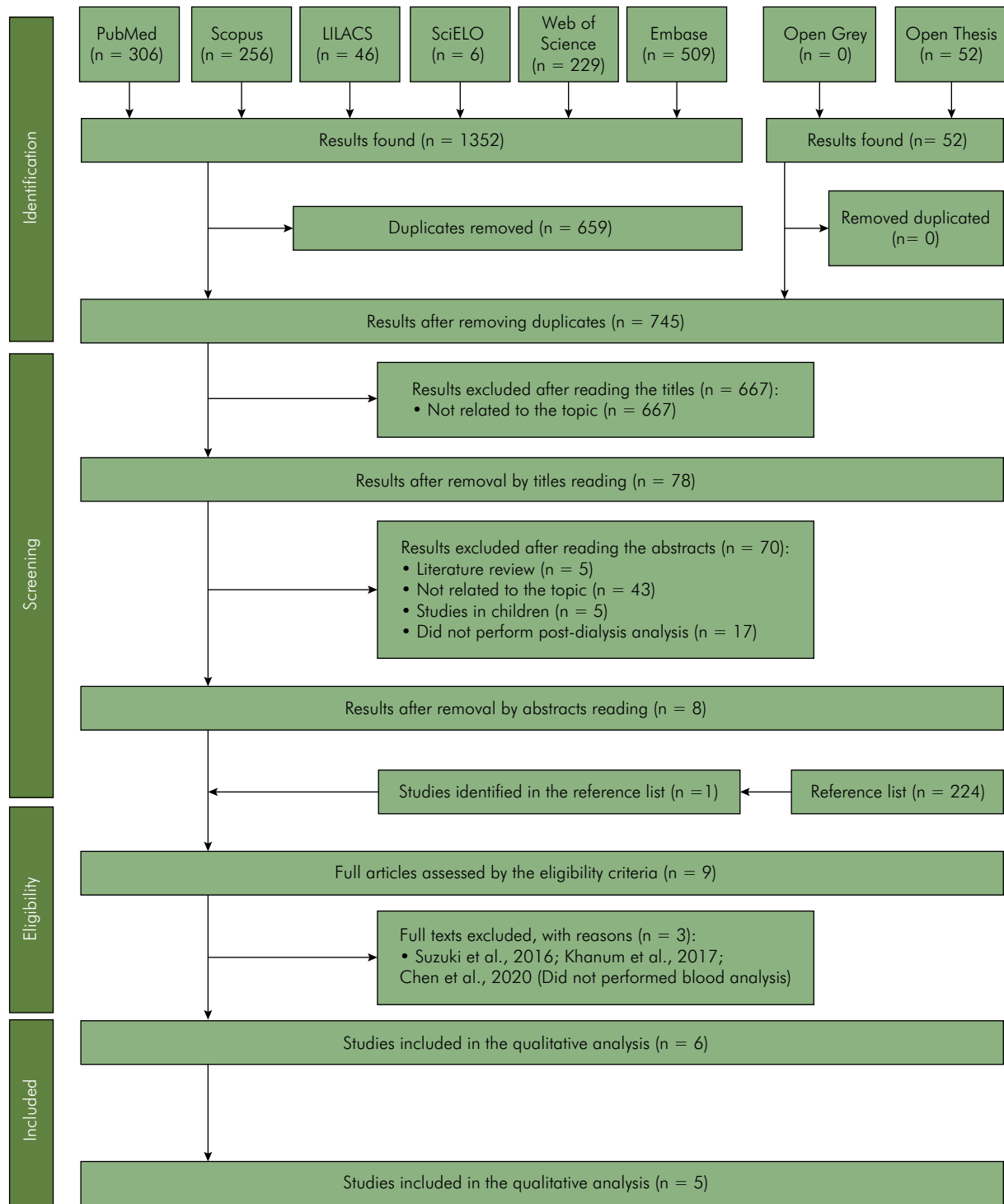
Figure 1. Flowchart of the literature search and selection process adapted from the PRISMA statement.
