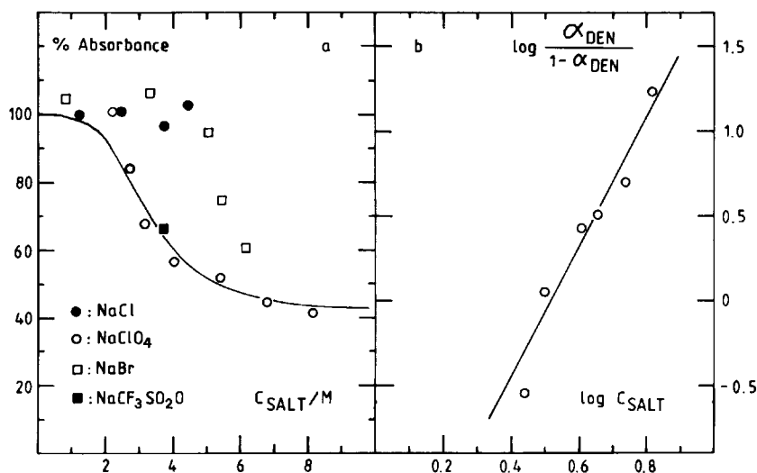
Fig. 7. Denaturation of equine metmyoglobin in aqueous sodium salt solutions with pH close to 7 (5 mM phosphate buffer) at 19°C as monitored by the decrease of the Soret absorption band ( \lambda_{\max} = 408 nm). (a) Absorbance (as percentage of absorbance in buffer without salt) as a function of salt concentration: Sodium chloride has no effect, even in a saturated sodium chloride solution, whereas sodium perchlorate has a transition point (concentration of denaturant required to effect 50% of the total change) at 3.3 M. Full line calculated for sodium perchlorate as denaturant using the parameters determined in part (b) of this figure. The transition caused by sodium bromide occurs at a higher concentration (above 5 M), although the limited solubility of sodium bromide hampers the exact determination. (b) Determination of K_{\text{DEN}} , the equilibrium constant for perchlorate denaturation of metmyoglobin, and n , the number of participating perchlorate ions according to eqn. (3): K_{\text{DEN}} = 0.011(7) and n = 3.8(4) .
