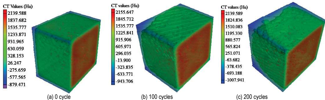
Figure 16 Distribution of CT values of concrete samples
