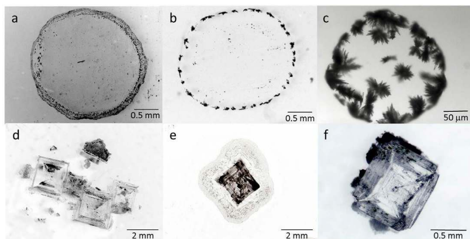
Figure 2. Crystallization pattern of two types of salt solution droplets at the end of drying on three types of glass slides with different wetting properties. Top panels (a,b,c): CaSO 4 ; bottom panels (d,e,f): NaCl. Left panels (a,d): Piranha cleaned; middle panels (b,e): Ehtanol+ Millipore water cleaned; right panels (c,f): silanized.
