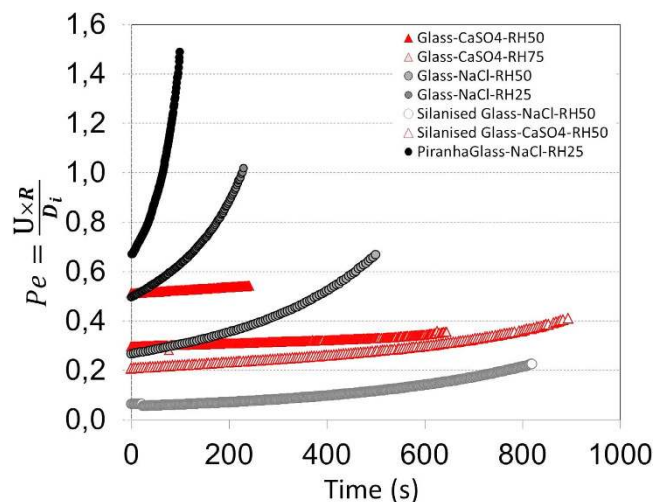
Figure 3. Peclet numbers calculated for droplets of 1\ \mu\text{l} size on cleaned glass slides (ethanol + water and Piranha) and silanized glass for the two different evaporation rates (see methods) till the precipitation of crystals in droplets.
