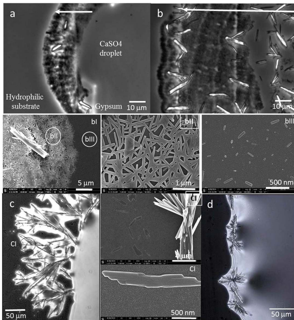
Figure 6. Phase-contrast and High resolution SEM micrographs of the growth of \text{CaSO}_4 polymorphs for various contact angles \theta of the droplet with the glass substrate. (a–b) \theta \sim 5^\circ : formation of an intermediate grey phase at the contact line followed by the spreading of the droplet with time (time between a and b images \sim 5 s). The arrow points are the spreading region from right to left. (bI–III) High-resolution SEM images of \text{CaSO}_4 crystals at the contact line of the droplet. Presence of nanorods and nanoparticles of bassanite and growth of gypsum from their assembly (Mikado-like structure) (c) \theta \sim 13^\circ : direct formation of gypsum needles in the bulk at the contact line region and spreading of the solution around the needles. (CI) High-resolution SEM images of \text{CaSO}_4 crystals at the contact line region, presence of nanocrystals of Gypsum (d) \theta \sim 30^\circ . clusters of interpenetrating gypsum needles (“sea urchin” shape) without the spreading of the droplet.
