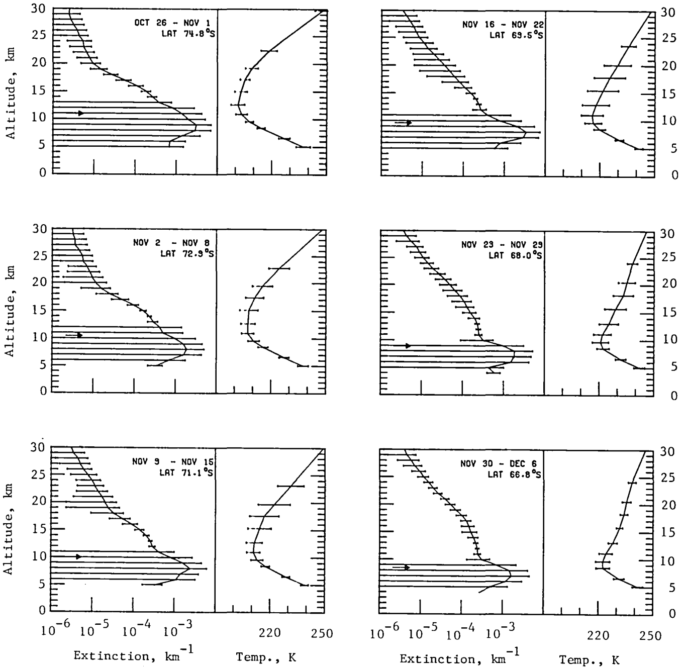
Figure 7.- Antarctic extinction and temperature profiles for October 26 to December 6, 1980.
