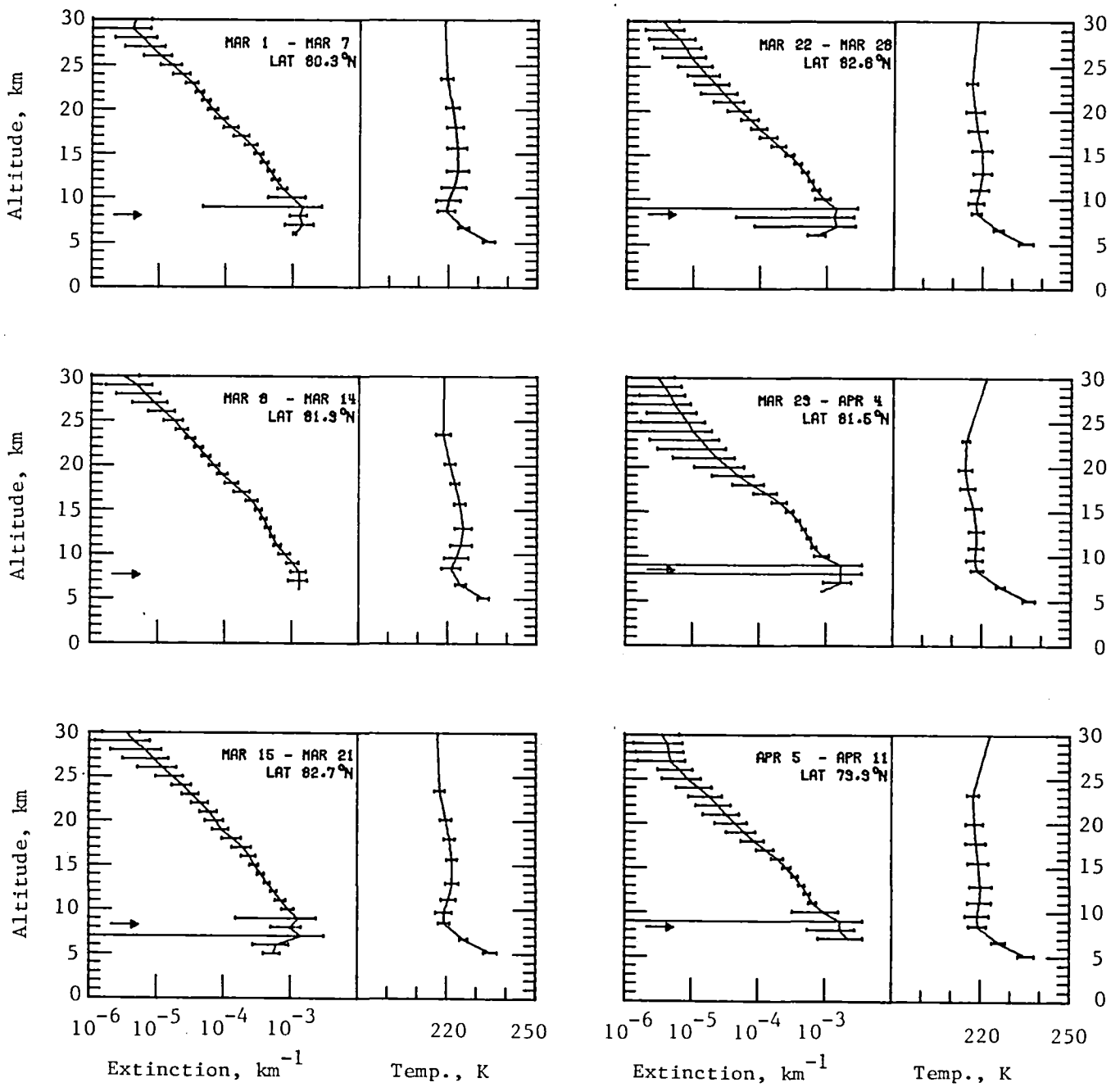
Figure 5.- Arctic extinction and temperature profiles for March 1 to April 11, 1981.
