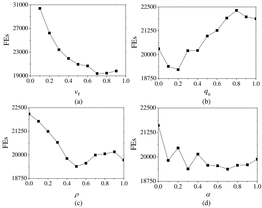
Fig. 7 Illustration of using different values of v_r, q_0, \rho, \alpha on f_6 . The y-axis represents the average number of FEs used for achieving an accuracy level smaller than \varepsilon = 1 , with the other parameters set as default.
