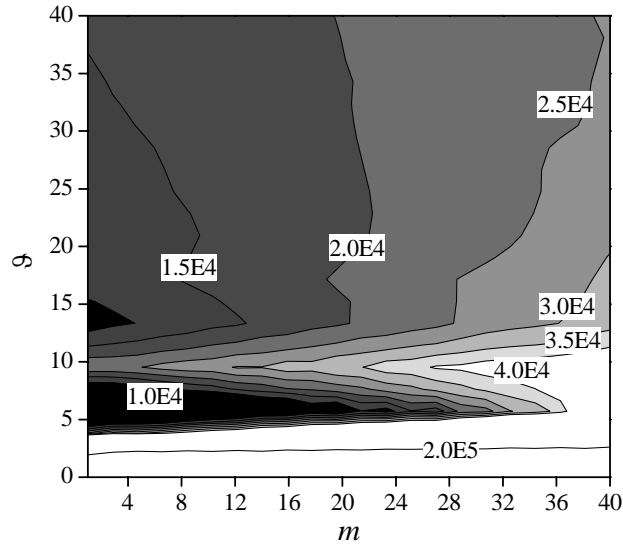
Fig. 6 Contour illustration of using different values of m and g on f_6 . The contour represents the average number of FEs used for achieving an accuracy level smaller than \varepsilon = 1 , with the other parameters set as default.
