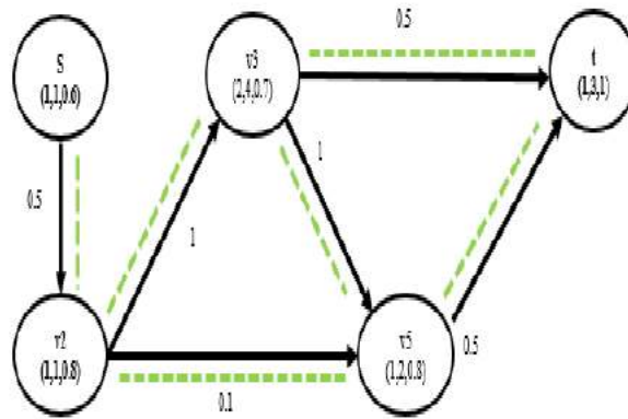
(c) Anypath representation from s to t (Path 2)
