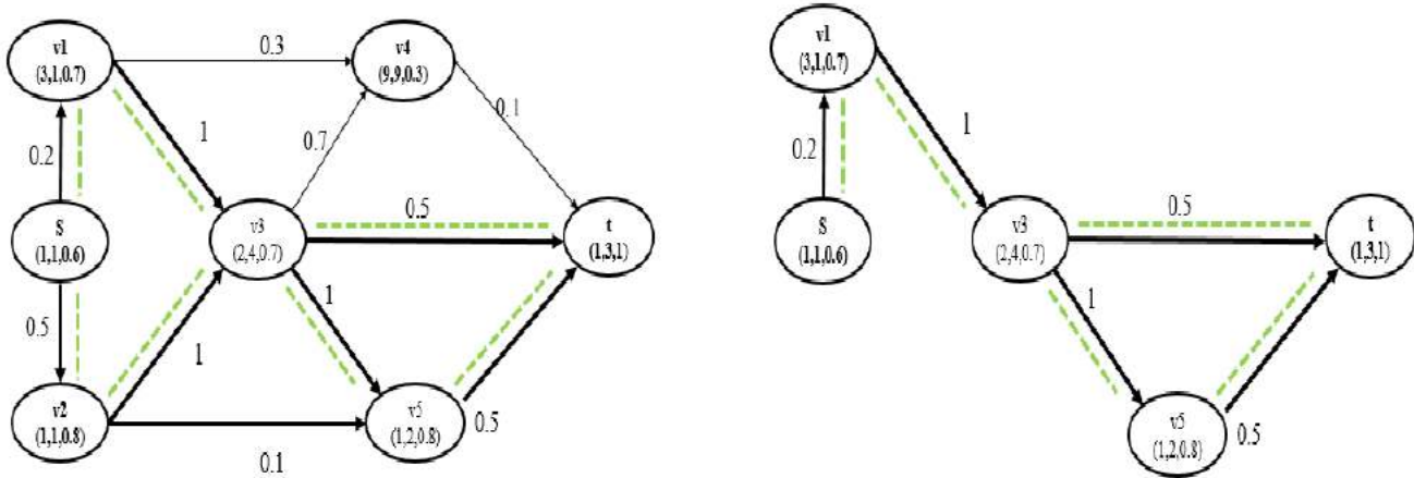
(a) Anypath representation for P_s
