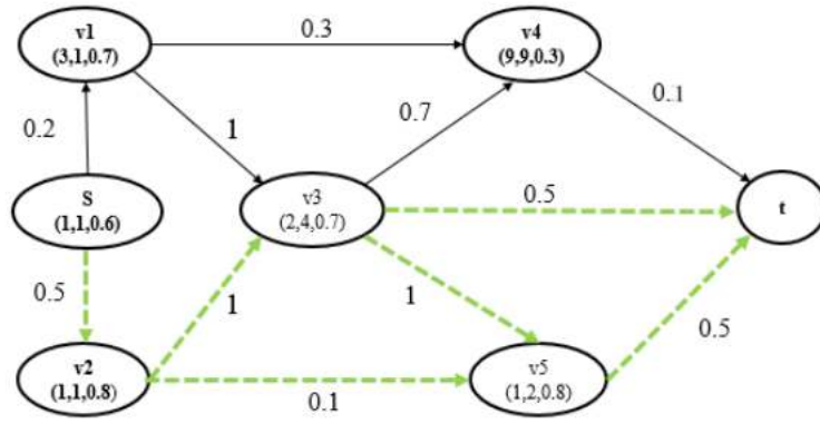
Fig. 3: Anypath Weight Computation
