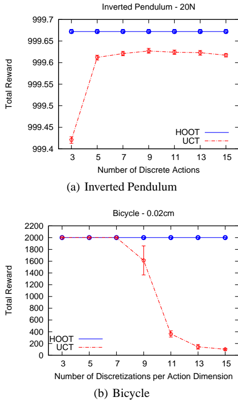
Figure 2: Performance of HOOT and UCT in two domains as the number of actions varies. The number of queries was fixed at 2048.
