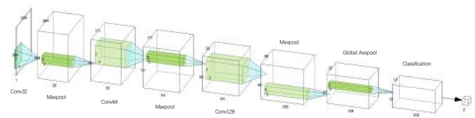
Fig. 3. CRNet architecture. Please zoom to view better
