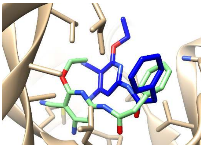
Figure S2. Orientation of the ligand in the binding pocket in two different windows during umbrella sampling simulations - i) Blue – window where the flexible bond is restrained to the same value as the stable pose, also the starting pose in the MD and MD/NCMC simulations. ii) Green – where the flexible bond is restrained to be at an angle of 90^\circ with respect to the starting orientation. The binding pose of the ligand gets altered in the second case. Hence, we decided to put additional positional restraints on the fixed part of the ligand in all of the windows to prevent the ligand from exploring other binding modes.
