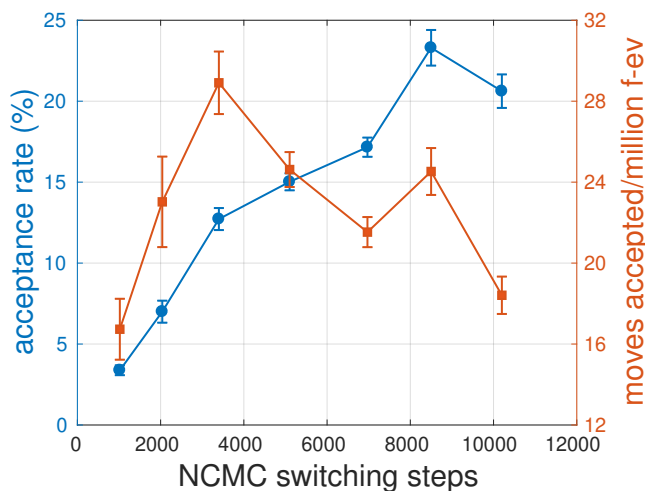
Figure 6. Acceptance rate of NCMC moves (in blue) and moves accepted per million force evaluations (f-ev) (in orange) as a function of the number of NCMC switching steps for ligand 1 . The acceptance rate increases with more NCMC steps. However, the number of moves accepted per million force evaluations initially increases and then decreases with the number of NCMC switching steps.
