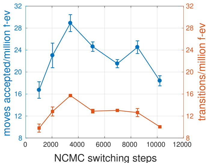
Figure S3. Moves accepted per million force evaluations (f-ev) during MD/NCMC simulation and transitions between different binding poses per million force evaluations (f-ev) as a function of the number of NCMC switching steps for ligand 1 . Accepted moves does not always result in a transition, as seen from the lower values of transitions/million f-ev.
