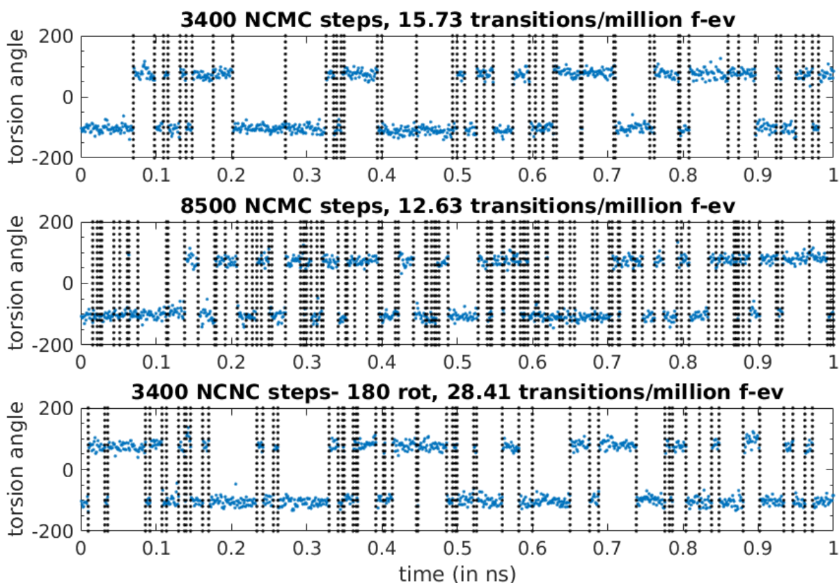
Figure S4. Torsion angles (corresponding to the two binding modes) as a function of time simulated with different NCMC protocols for ligand 1 - 3400 NCMC steps ( top ) and 8500 NCMC steps ( middle ) with random rotational moves; 3400 NCMC steps with random 180° rotational moves ( bottom ). Black dotted vertical lines show the accepted NCMC moves. Not all accepted moves result in a transition between the two binding modes for random rotational moves. For example, during the first 0.1 ns of NCMC simulation in middle , moves were accepted, but did not correspond to a successful transition. However, with 180° rotational moves, almost every accepted move resulted in a transition with almost two times increase in the transitions per million force evaluations (transitions/million f-ev).
