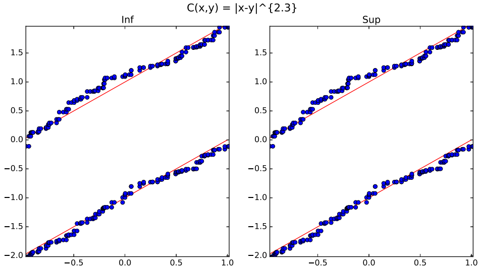
FIGURE 2. Points (x_i, y_j) such that r_{ij}^* > 0 , where r^* is the optimal solution of the MOT minimization (1.1) with c(x, y) = |y - x|^{2.3} for (\tilde{\mu}_I \wedge \tilde{\nu}_I, \tilde{\nu}_I) at left and (\tilde{\mu}_I, \tilde{\mu}_I \vee \tilde{\nu}_I) at right, with I = 100 . The segments y = x \pm 1 , x \in [-1, 1] indicate the support of \pi^* given by (6.1).
