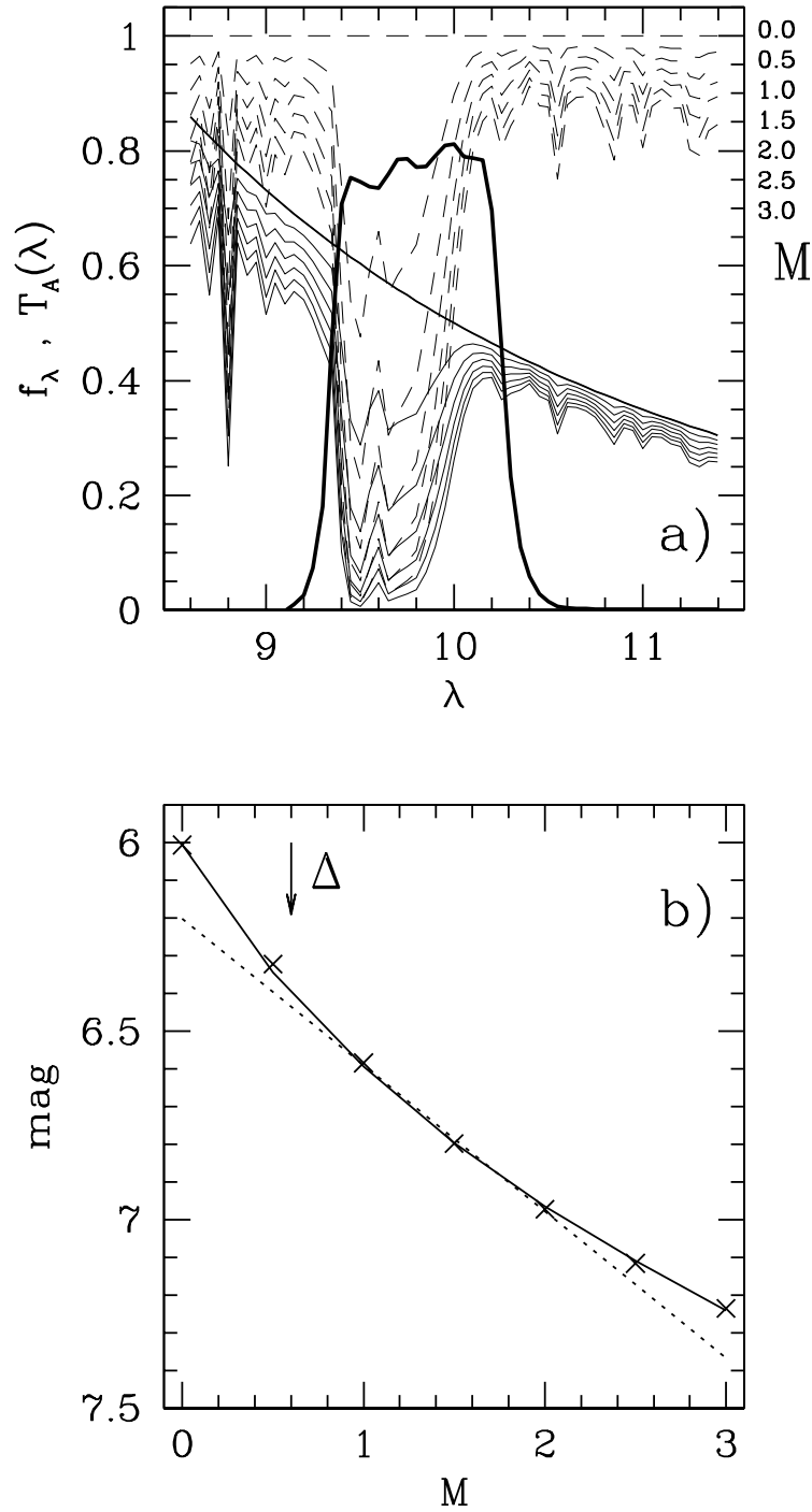
Fig. 2. Forbes effect. (a) Atmospheric transmission T_A(\lambda) (dashed line) for increasing air-mass M from 0 to 3, attenuates an observed continuum source f_\lambda (thin lines). The spectral region corresponds to the SiP filter (solid line). (b) Magnitude obtained by integrating the transmitted flux over the filter's response (crosses) for each air-mass M . An error \Delta is made from the extrapolation of a linear (Bouguer) extinction law (dotted line). A fit by Padé approximants (solid line) may correct this problem.
