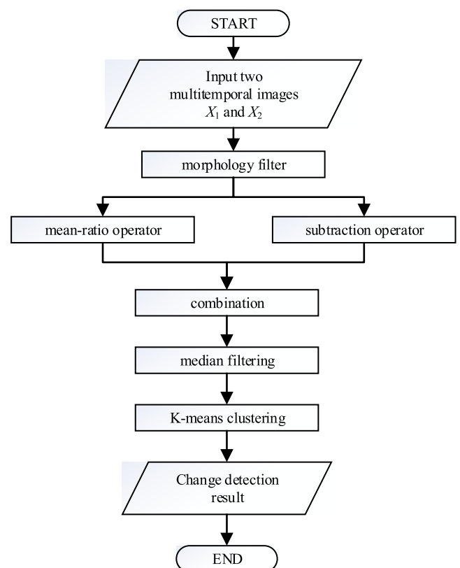
FIGURE 1. Algorithm flowchart.
