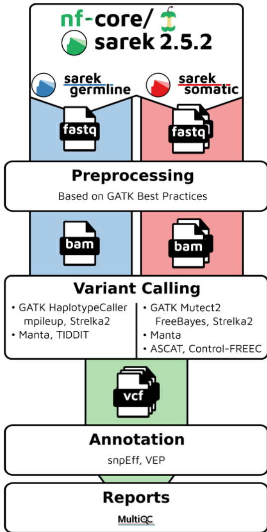
Figure 1. Schematic overview of the Sarek workflow for analysis of germline and somatic variants. A schematic overview including some of the main analysis software implemented in the Sarek workflow. A more comprehensive list of the currently implemented software is given in Table 1 .
