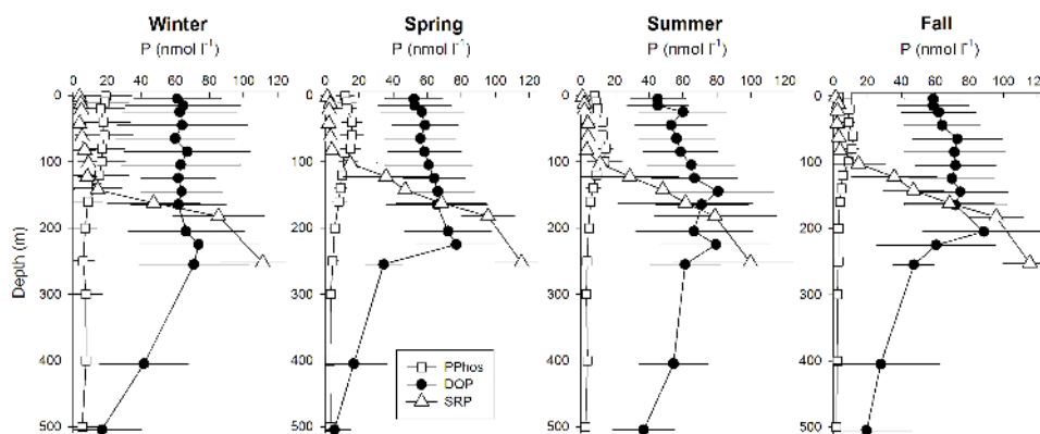
Fig. 1. Seasonal mean (+stdev) profiles of PPhos (squares), DOP (filled circles), and MAGIC-SRP (open triangles) at BATS. All concentrations are in \text{nmol l}^{-1} . n = 6\text{--}15 for each depth depending upon season and phosphorus pool. Depths are slightly offset such that error bars do not overlap.
