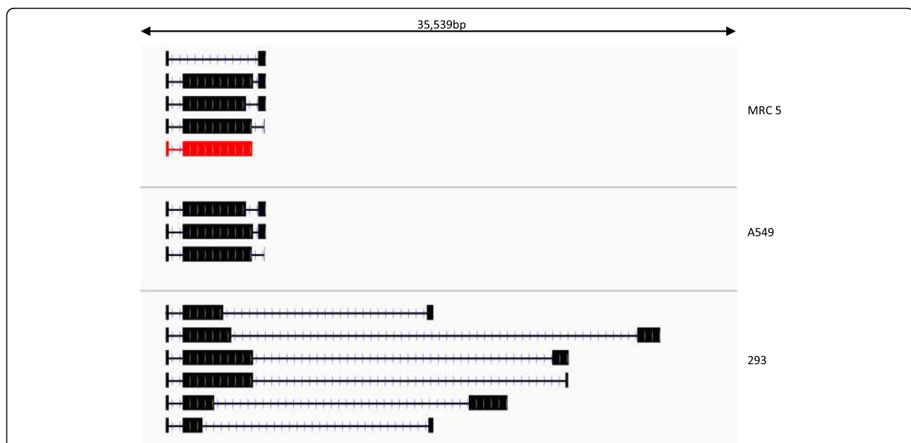
Fig. 2 Transcript heterogeneity. This figure illustrates the structure of various transcripts observed at very low levels (less than 10 transcripts per dataset) all of which initiate at the transcription start site that drives expression of the S glycoprotein. For orientation, the structure of the dominant S glycoprotein transcript is shown in red in the examples selected from the MRC5 dataset. Three sets of example transcripts are shown from MRC5, A549 and HEK293 cells. The transcripts shown arise from splicing events that utilise only the canonical GU-AG splice donor/acceptor pair present in over 90% of eukaryotic splicing events. As can be seen, some of the transcripts arise from unintended splice site usage as well as from missing the intended BGH polyadenylation signal and utilising other polyadenylation signals further down the vector genome
