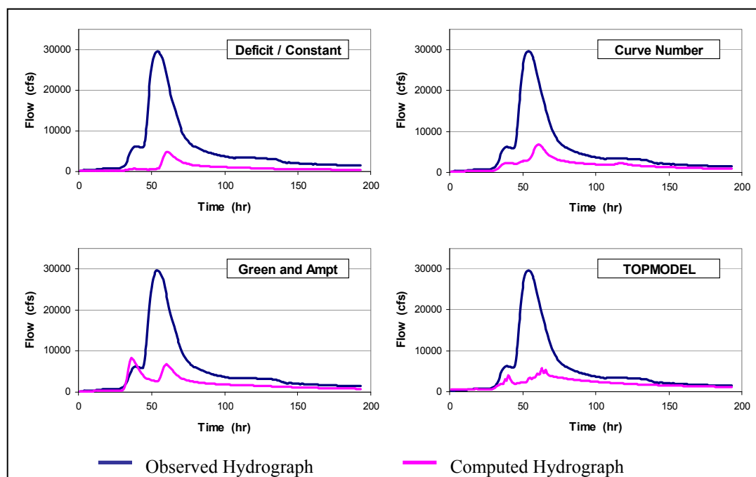
Figure 5. Computed vs. Observed Hydrographs using actual satellite rainfall data (unadjusted) at the native scale of 0.25^\circ .
