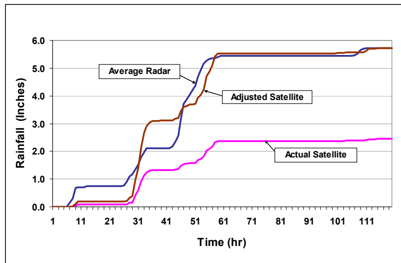
Figure 6. Cumulative satellite rainfall hyetographs for deriving bias adjustment.
