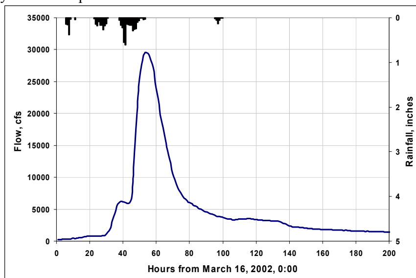
Figure 3. Rainfall and runoff for the March 2002 storm event.
