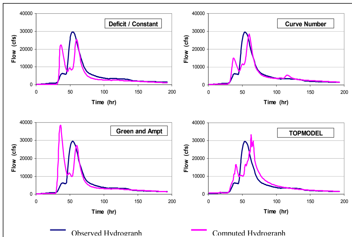
Figure 7. Computed vs. Observed Hydrographs using actual satellite rainfall data (adjusted) at the native scale of 0.25^\circ .
