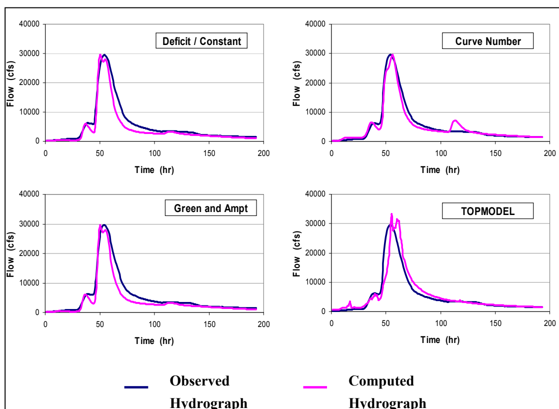
Figure 4. Observed versus simulated stream flow for four hydrologic model configurations in the UC river basin ( taken from Harris, 2007 ). Note: Other than TOPMODEL, all other configurations shown above can be set up in HEC-HMS.
