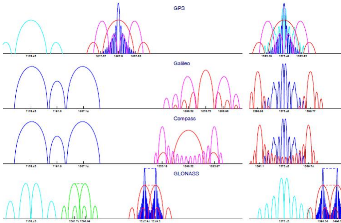
Figure 1: Signal Spectra for GPS, Galileo, Compass and GLONASS. From the left, new GPS satellites radiate at L5 (1176.45 MHz), L2 (1227.60 MHz) and L1 (1575.42 MHz). (From Liang Heng)
