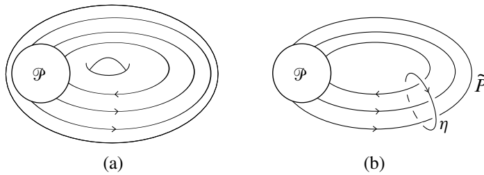
Figure 3: (a) A schematic picture of a pattern P . The circle containing \mathcal{P} denotes a tangle. (b) The 2-component link corresponding to the pattern P . The circle containing \mathcal{P} denotes the same tangle as in the previous panel.
