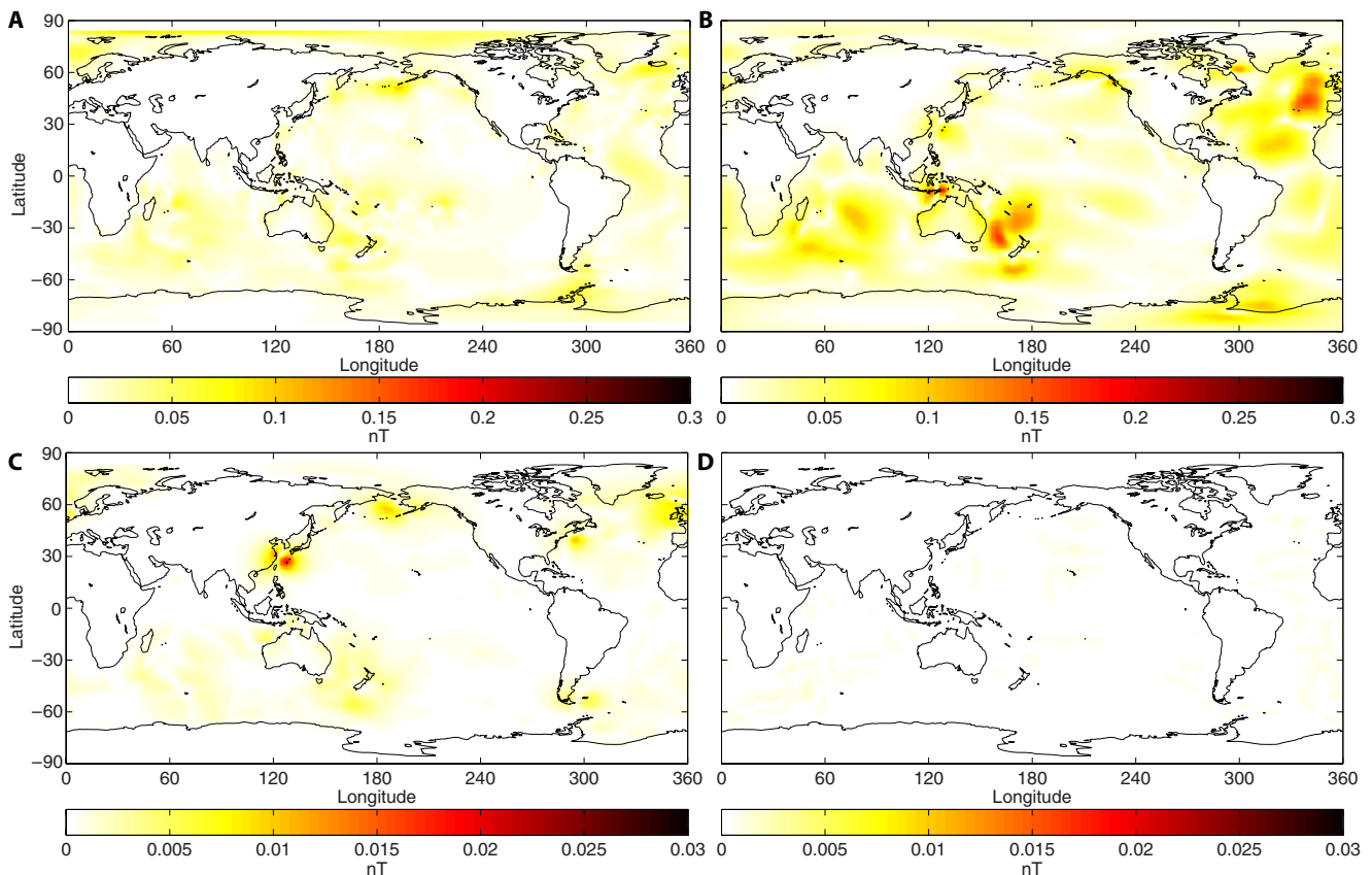
Fig. 5. Testing the sensitivity of the modeled responses to uncertainty in the extraneous current j^{ext} term. The amplitude difference of the radial magnetic field component between models using extraneous current constructed with (A) TPX08-atlas and HAMTIDE tidal models, (B) a constant ocean electrical conductivity of 3.2 S/m and LVOC shown in Fig. 1D, (C) seasonally averaged conductivity (Fig. 1D) and Northern Hemisphere winter ocean conductivity, and (D) core field and core plus lithosphere fields. All fields are calculated at an altitude of 430 km. The recovered structurally sparse model (Fig. 4) was used as a mantle conductivity profile for these tests. Note the different scales.
